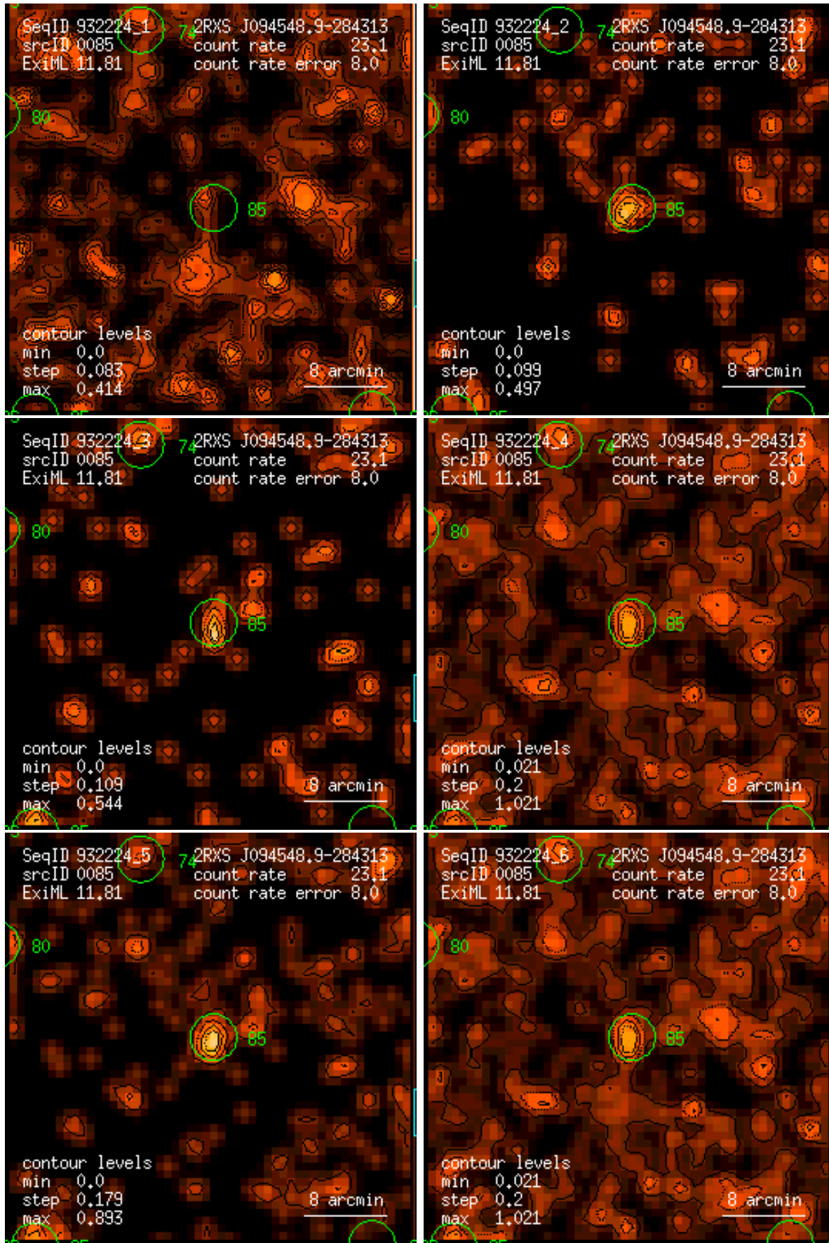
Figure 85: RASS 932224: detection 0085: band rate images, Gaussian filter: (1) PSPC channels 11 – 41, (2) 52 – 90, (3) 91 – 201, (4) 11 – 235, (5) 52 – 201, (6) 11 – 201. Broad band rates in counts/ks. Band rate contour levels in counts/ks/arcmin 2 .
