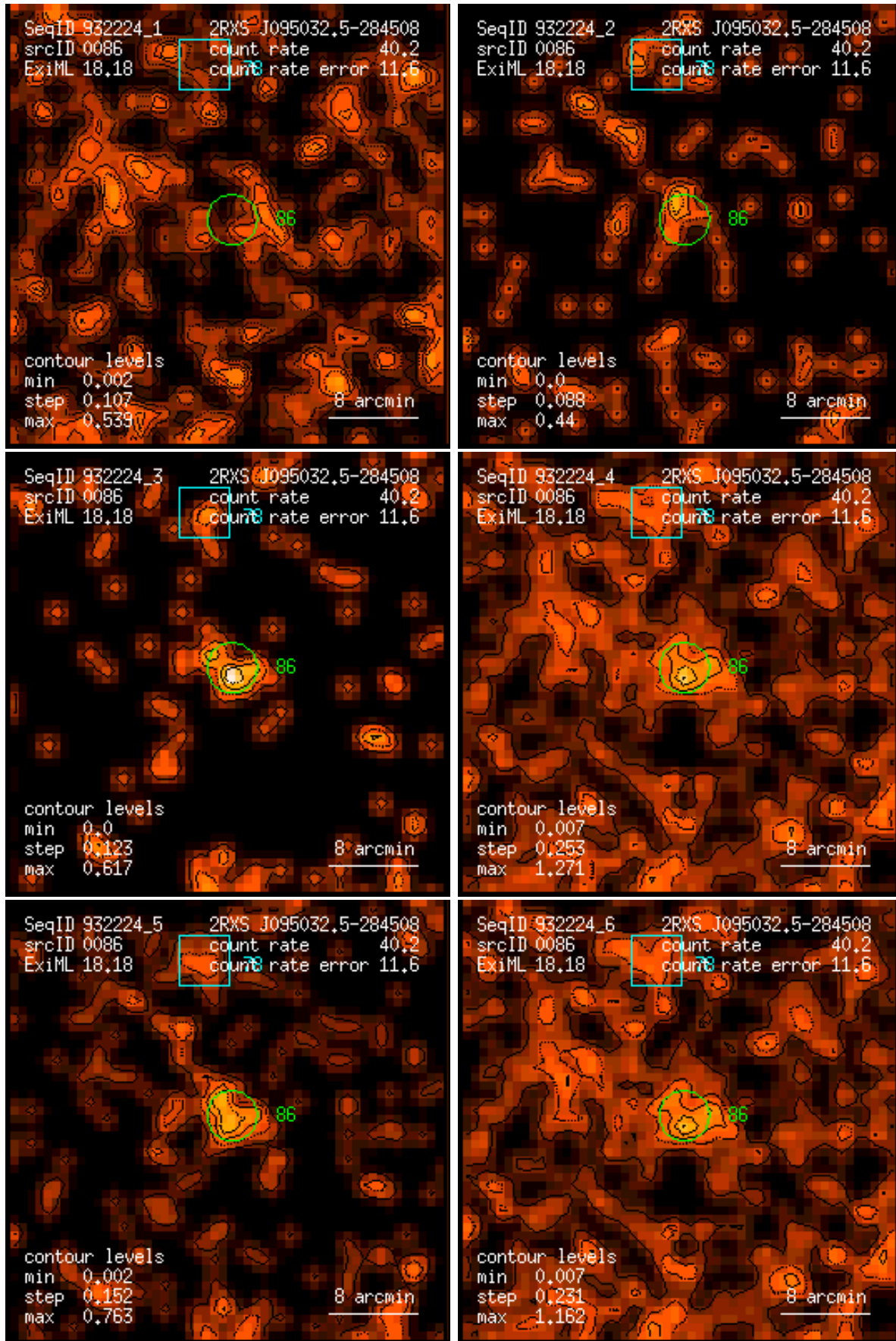
Figure 86: RASS 932224: detection 0086: band rate images, Gaussian filter: (1) PSPC channels 11 – 41, (2) 52 – 90, (3) 91 – 201, (4) 11 – 235, (5) 52 – 201, (6) 11 – 201. Broad band rates in counts/ks. Band rate contour levels in counts/ks/arcmin 2 .
