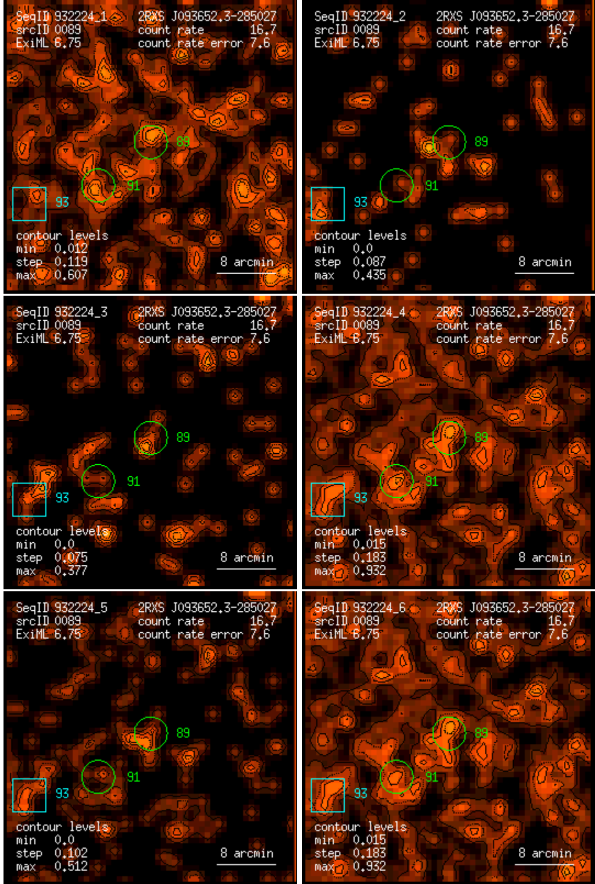
Figure 89: RASS 932224: detection 0089: band rate images, Gaussian filter: (1) PSPC channels 11 – 41, (2) 52 – 90, (3) 91 – 201, (4) 11 – 235, (5) 52 – 201, (6) 11 – 201. Broad band rates in counts/ks. Band rate contour levels in counts/ks/arcmin 2 .
