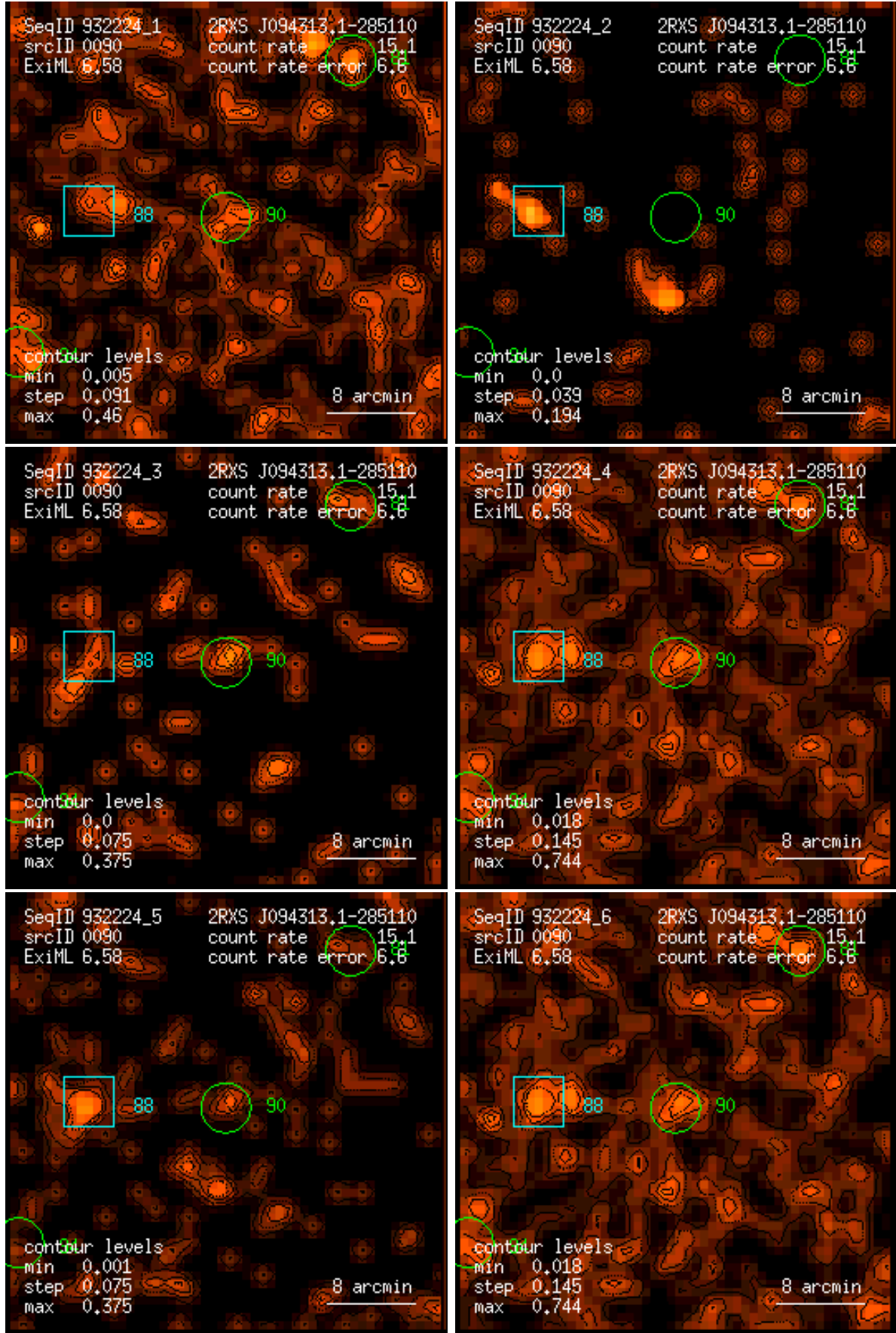
Figure 90: RASS 932224: detection 0090: band rate images, Gaussian filter: (1) PSPC channels 11 – 41, (2) 52 – 90, (3) 91 – 201, (4) 11 – 235, (5) 52 – 201, (6) 11 – 201. Broad band rates in counts/ks. Band rate contour levels in counts/ks/arcmin 2 .
