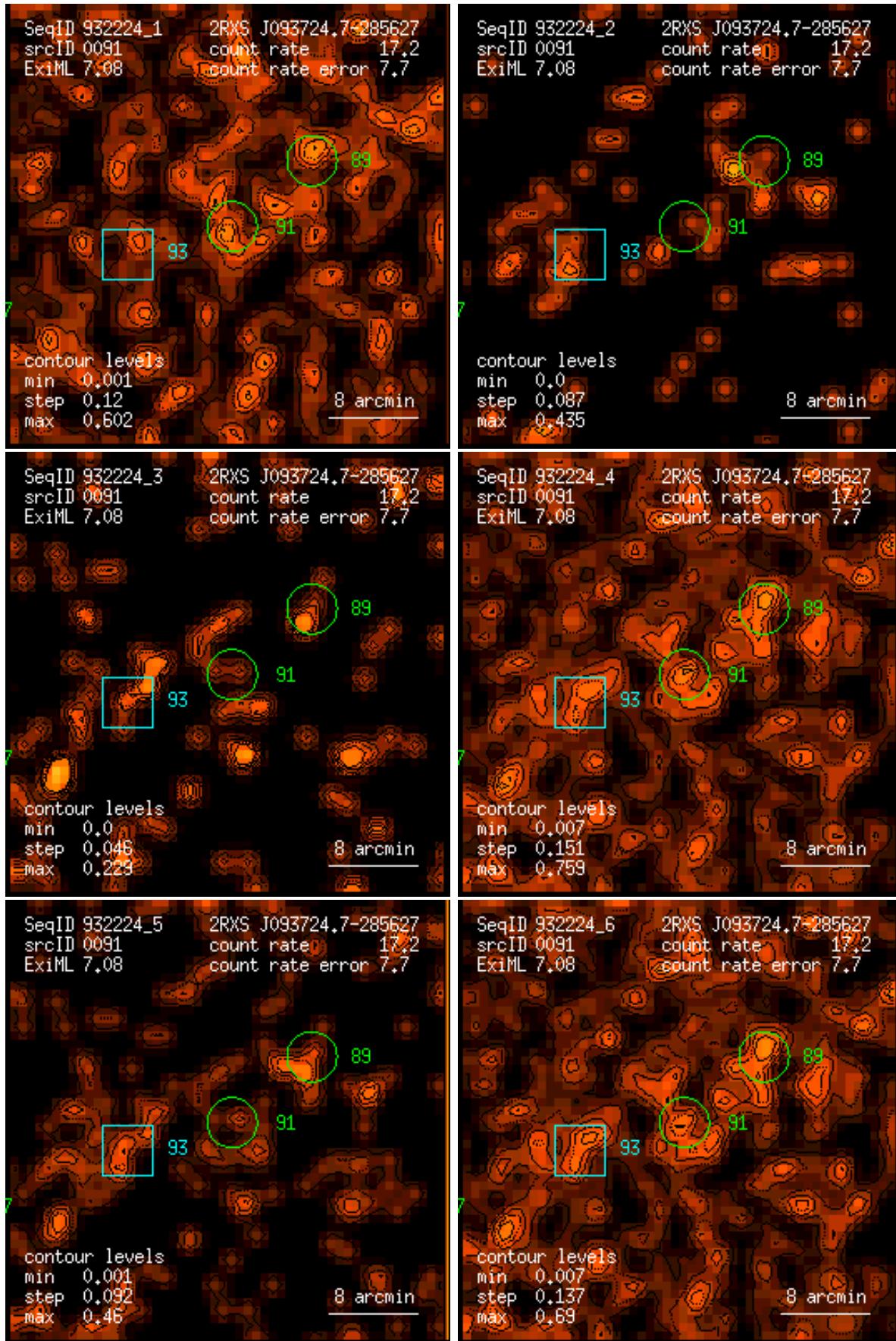
Figure 91: RASS 932224: detection 0091: band rate images, Gaussian filter: (1) PSPC channels 11 – 41, (2) 52 – 90, (3) 91 – 201, (4) 11 – 235, (5) 52 – 201, (6) 11 – 201. Broad band rates in counts/ks. Band rate contour levels in counts/ks/arcmin 2 .
