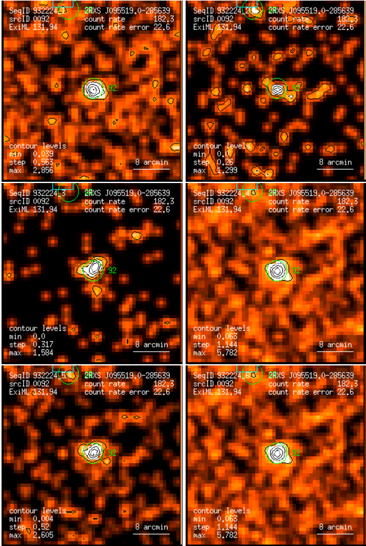
Figure 92: RASS 932224: detection 0092: band rate images, Gaussian filter: (1) PSPC channels 11 – 41, (2) 52 – 90, (3) 91 – 201, (4) 11 – 235, (5) 52 – 201, (6) 11 – 201. Broad band rates in counts/ks. Band rate contour levels in counts/ks/arcmin 2 .
