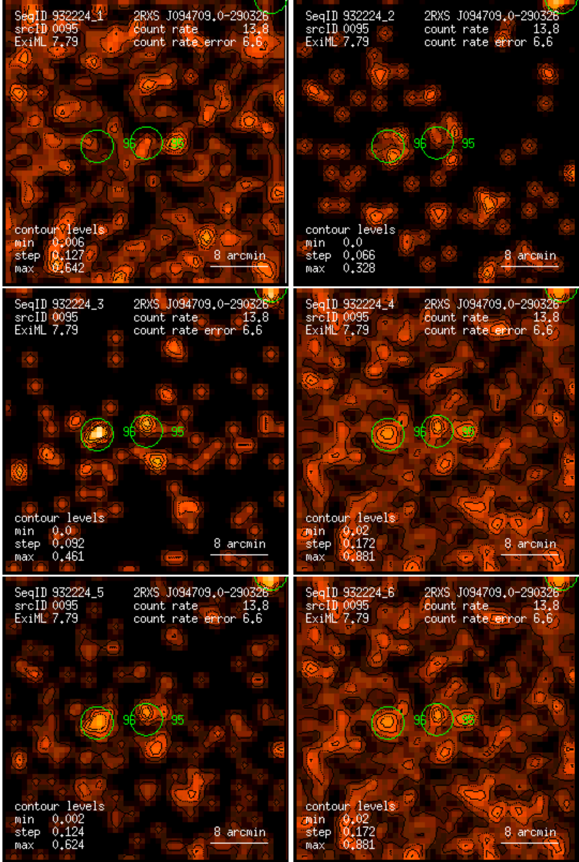
Figure 95: RASS 932224: detection 0095: band rate images, Gaussian filter: (1) PSPC channels 11 – 41, (2) 52 – 90, (3) 91 – 201, (4) 11 – 235, (5) 52 – 201, (6) 11 – 201. Broad band rates in counts/ks. Band rate contour levels in counts/ks/arcmin 2 .
