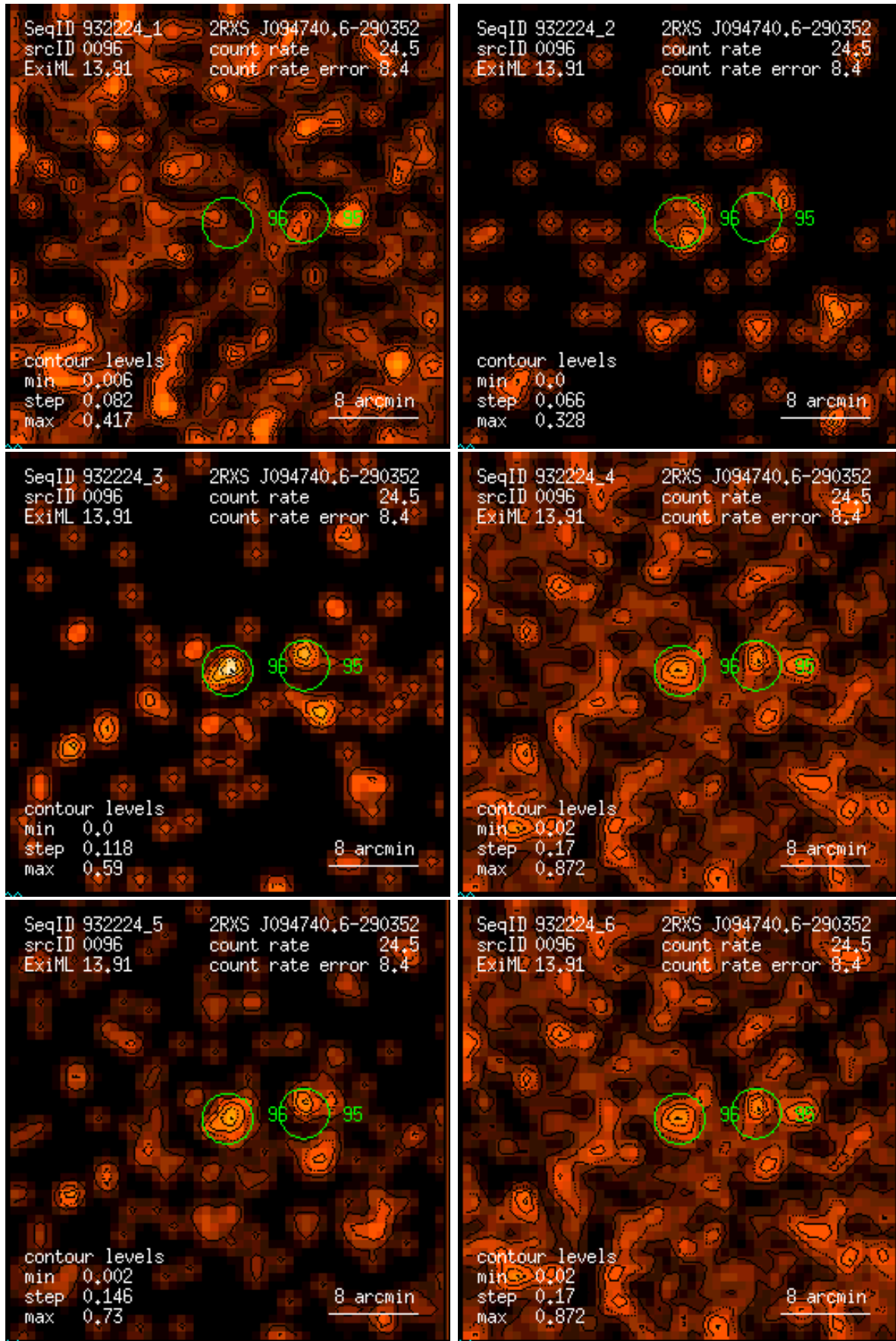
Figure 96: RASS 932224: detection 0096: band rate images, Gaussian filter: (1) PSPC channels 11 – 41, (2) 52 – 90, (3) 91 – 201, (4) 11 – 235, (5) 52 – 201, (6) 11 – 201. Broad band rates in counts/ks. Band rate contour levels in counts/ks/arcmin 2 .
