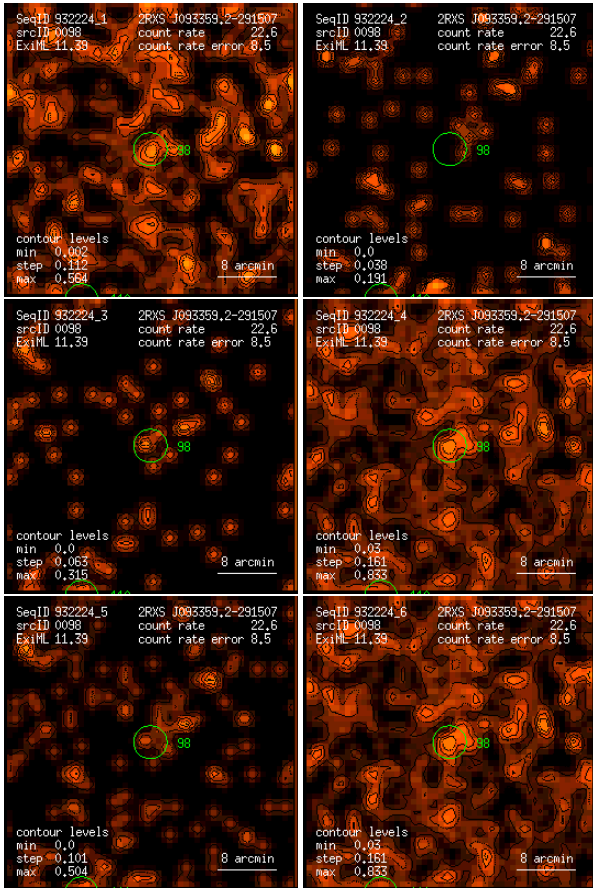
Figure 98: RASS 932224: detection 0098: band rate images, Gaussian filter: (1) PSPC channels 11 – 41, (2) 52 – 90, (3) 91 – 201, (4) 11 – 235, (5) 52 – 201, (6) 11 – 201. Broad band rates in counts/ks. Band rate contour levels in counts/ks/arcmin 2 .
