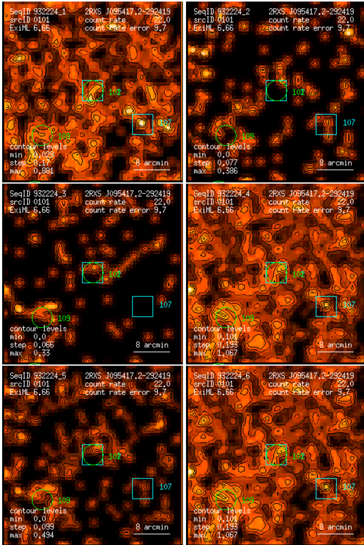
Figure 101: RASS 932224: detection 0101: band rate images, Gaussian filter: (1) PSPC channels 11 – 41, (2) 52 – 90, (3) 91 – 201, (4) 11 – 235, (5) 52 – 201, (6) 11 – 201. Broad band rates in counts/ks. Band rate contour levels in counts/ks/arcmin 2 .
