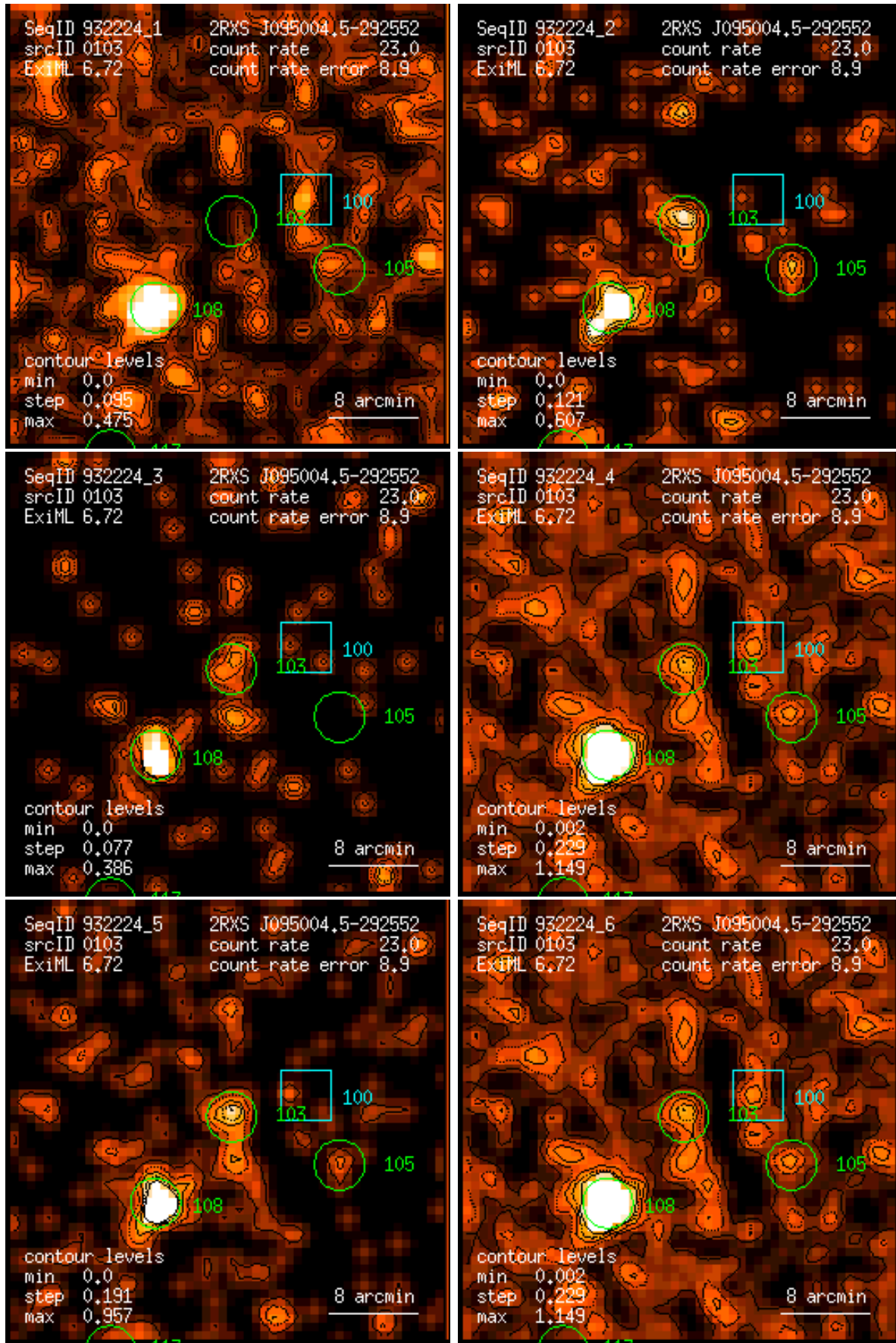
Figure 103: RASS 932224: detection 0103: band rate images, Gaussian filter: (1) PSPC channels 11 – 41, (2) 52 – 90, (3) 91 – 201, (4) 11 – 235, (5) 52 – 201, (6) 11 – 201. Broad band rates in counts/ks. Band rate contour levels in counts/ks/arcmin 2 .
