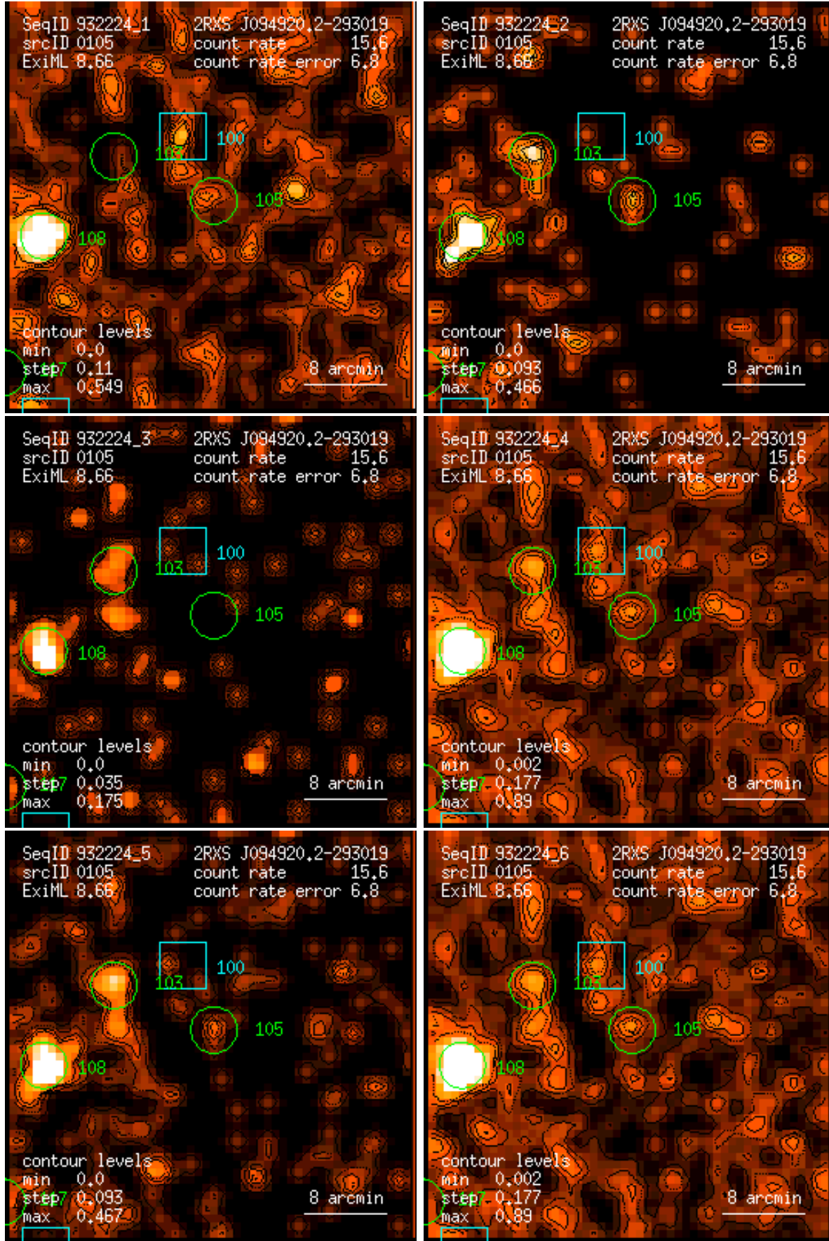
Figure 105: RASS 932224: detection 0105: band rate images, Gaussian filter: (1) PSPC channels 11 – 41, (2) 52 – 90, (3) 91 – 201, (4) 11 – 235, (5) 52 – 201, (6) 11 – 201. Broad band rates in counts/ks. Band rate contour levels in counts/ks/arcmin 2 .
