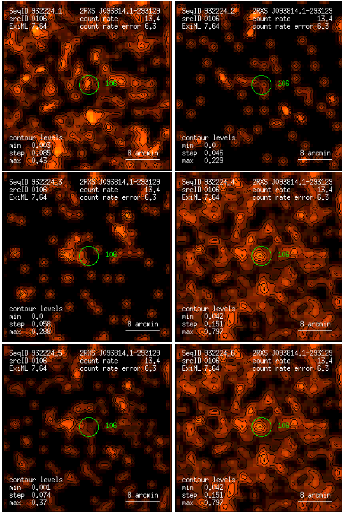
Figure 106: RASS 932224: detection 0106: band rate images, Gaussian filter: (1) PSPC channels 11 – 41, (2) 52 – 90, (3) 91 – 201, (4) 11 – 235, (5) 52 – 201, (6) 11 – 201. Broad band rates in counts/ks. Band rate contour levels in counts/ks/arcmin 2 .
