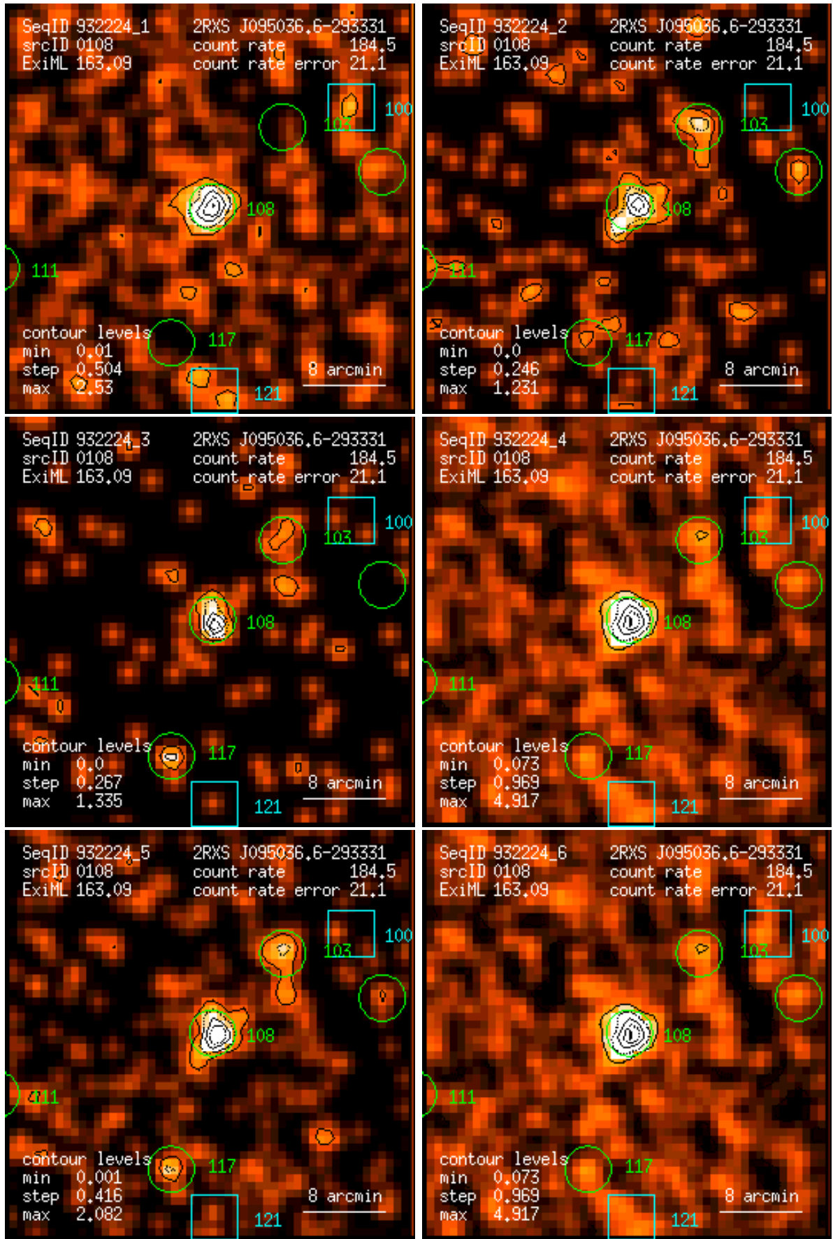
Figure 108: RASS 932224: detection 0108: band rate images, Gaussian filter: (1) PSPC channels 11 – 41, (2) 52 – 90, (3) 91 – 201, (4) 11 – 235, (5) 52 – 201, (6) 11 – 201. Broad band rates in counts/ks. Band rate contour levels in counts/ks/arcmin 2 .
