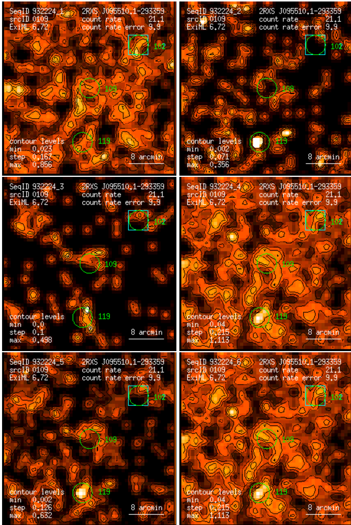
Figure 109: RASS 932224: detection 0109: band rate images, Gaussian filter: (1) PSPC channels 11 – 41, (2) 52 – 90, (3) 91 – 201, (4) 11 – 235, (5) 52 – 201, (6) 11 – 201. Broad band rates in counts/ks. Band rate contour levels in counts/ks/arcmin 2 .
