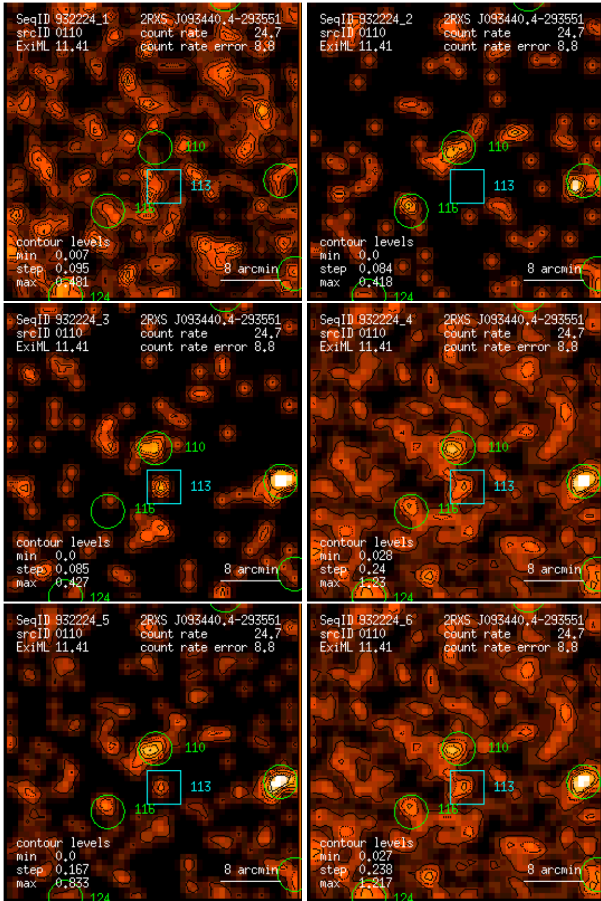
Figure 110: RASS 932224: detection 0110: band rate images, Gaussian filter: (1) PSPC channels 11 – 41, (2) 52 – 90, (3) 91 – 201, (4) 11 – 235, (5) 52 – 201, (6) 11 – 201. Broad band rates in counts/ks. Band rate contour levels in counts/ks/arcmin 2 .
