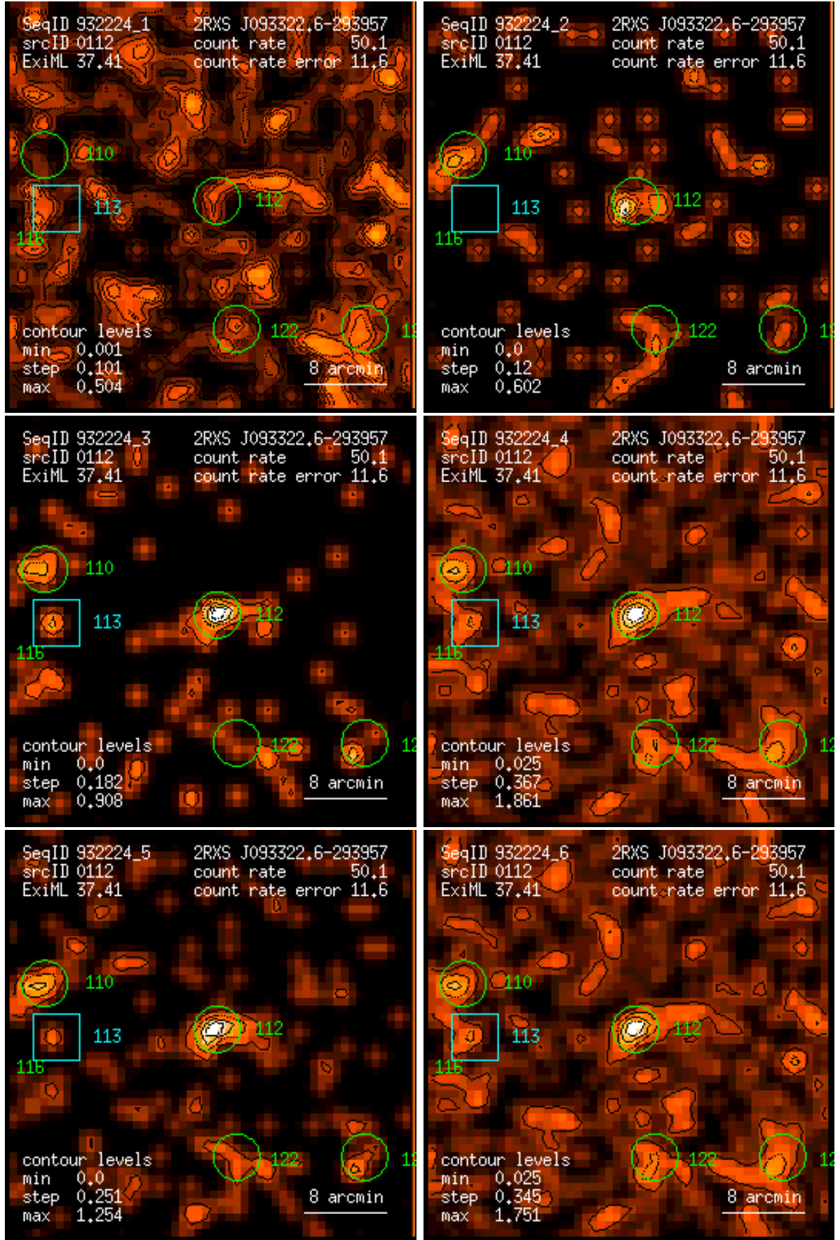
Figure 112: RASS 932224: detection 0112: band rate images, Gaussian filter: (1) PSPC channels 11 – 41, (2) 52 – 90, (3) 91 – 201, (4) 11 – 235, (5) 52 – 201, (6) 11 – 201. Broad band rates in counts/ks. Band rate contour levels in counts/ks/arcmin 2 .
