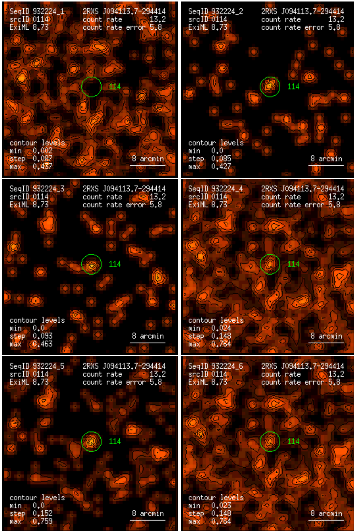
Figure 114: RASS 932224: detection 0114: band rate images, Gaussian filter: (1) PSPC channels 11 – 41, (2) 52 – 90, (3) 91 – 201, (4) 11 – 235, (5) 52 – 201, (6) 11 – 201. Broad band rates in counts/ks. Band rate contour levels in counts/ks/arcmin 2 .
