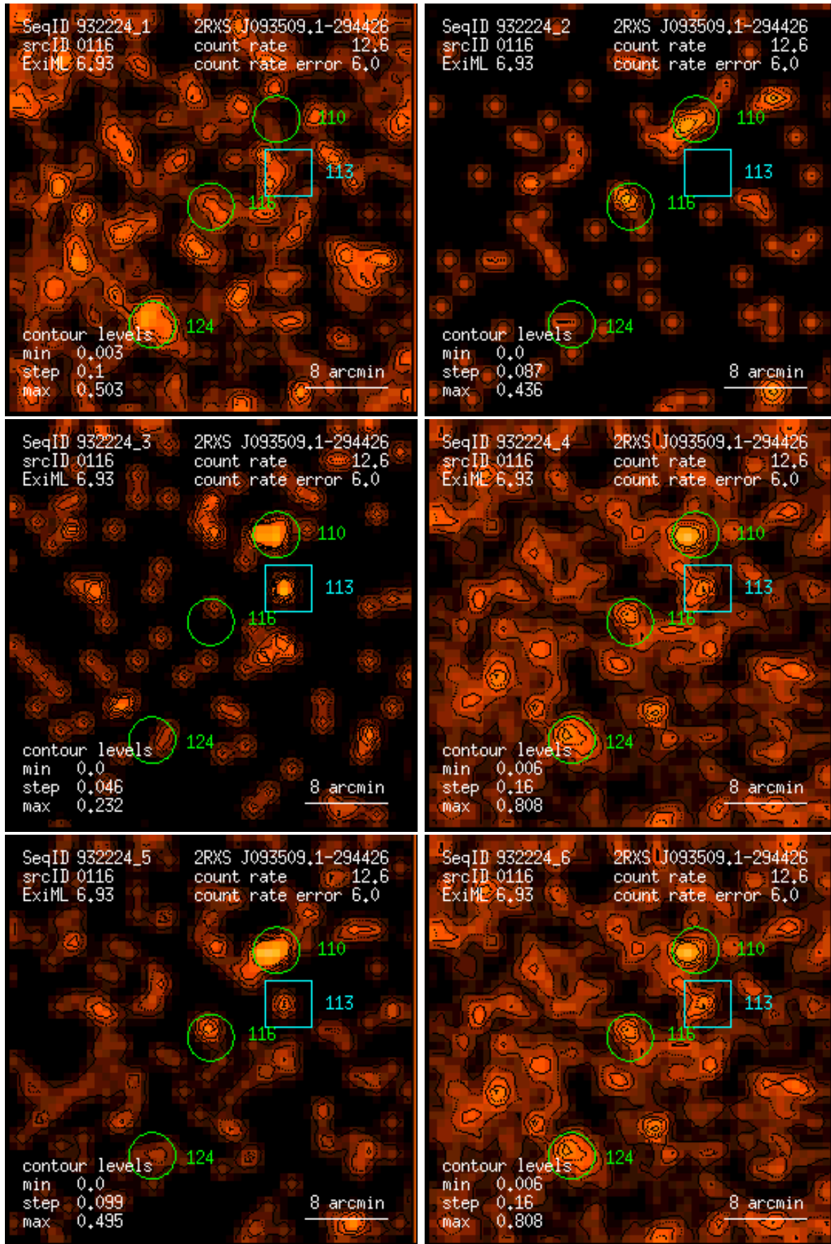
Figure 116: RASS 932224: detection 0116: band rate images, Gaussian filter: (1) PSPC channels 11 – 41, (2) 52 – 90, (3) 91 – 201, (4) 11 – 235, (5) 52 – 201, (6) 11 – 201. Broad band rates in counts/ks. Band rate contour levels in counts/ks/arcmin 2 .
