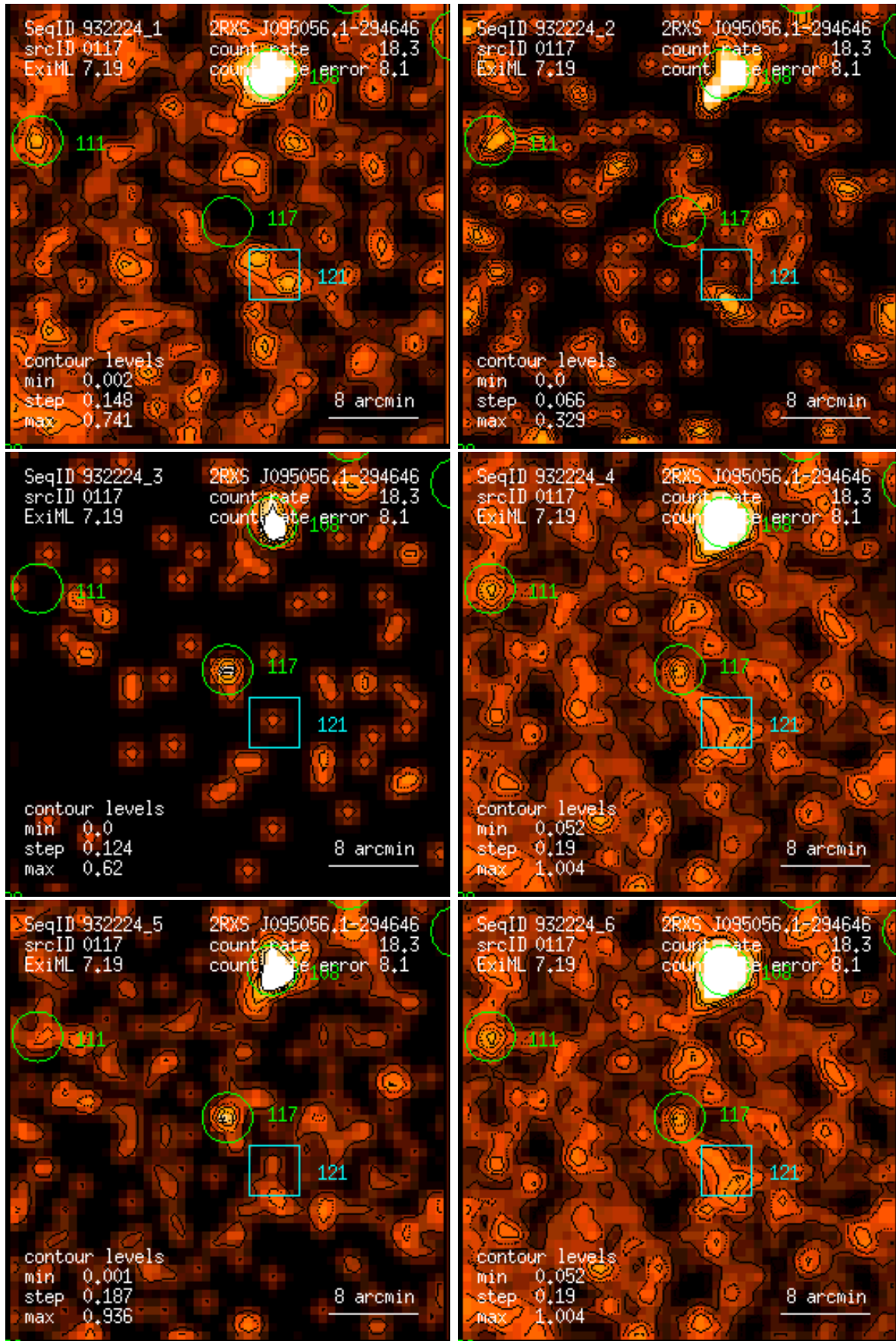
Figure 117: RASS 932224: detection 0117: band rate images, Gaussian filter: (1) PSPC channels 11 – 41, (2) 52 – 90, (3) 91 – 201, (4) 11 – 235, (5) 52 – 201, (6) 11 – 201. Broad band rates in counts/ks. Band rate contour levels in counts/ks/arcmin 2 .
