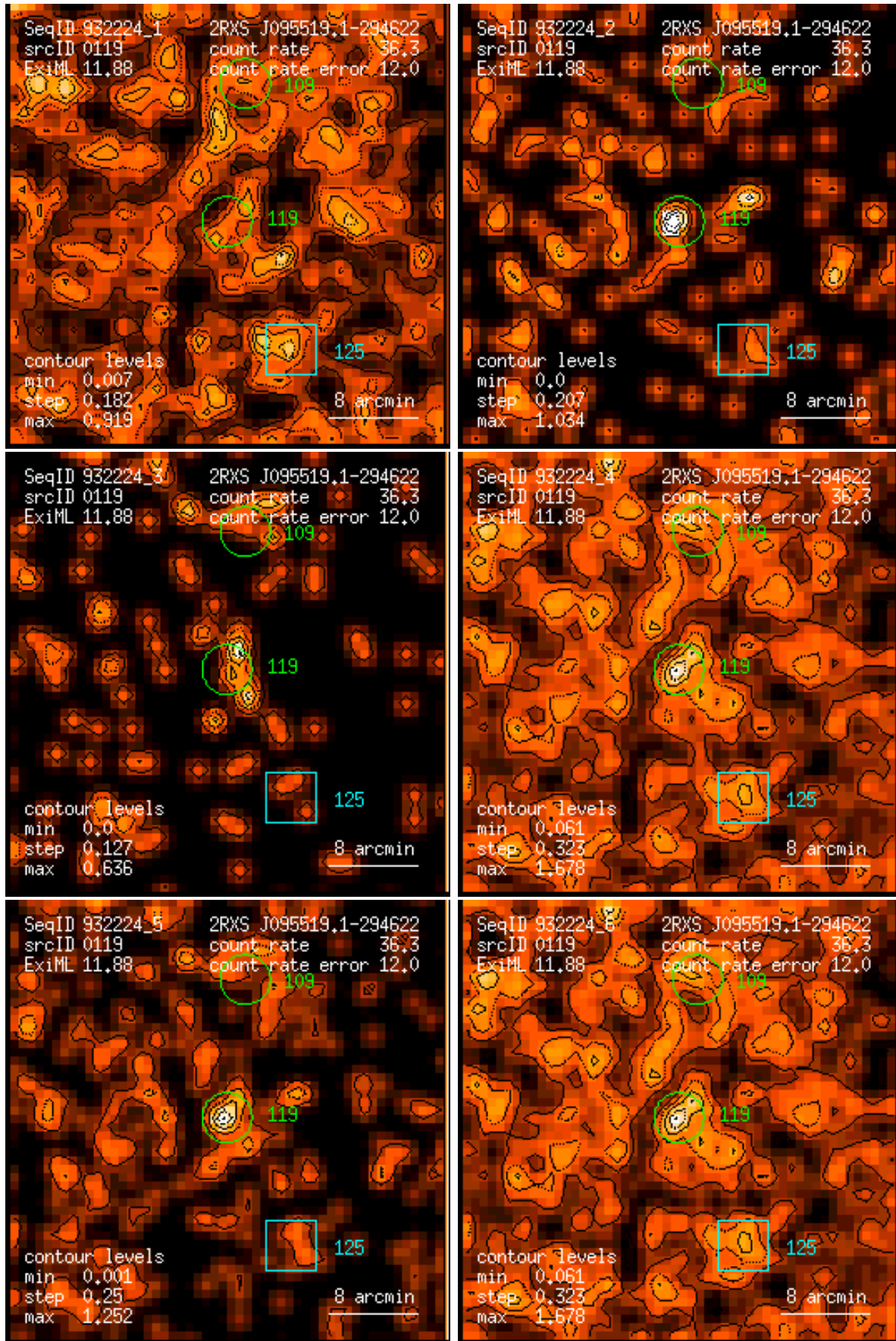
Figure 119: RASS 932224: detection 0119: band rate images, Gaussian filter: (1) PSPC channels 11 – 41, (2) 52 – 90, (3) 91 – 201, (4) 11 – 235, (5) 52 – 201, (6) 11 – 201. Broad band rates in counts/ks. Band rate contour levels in counts/ks/arcmin 2 .
