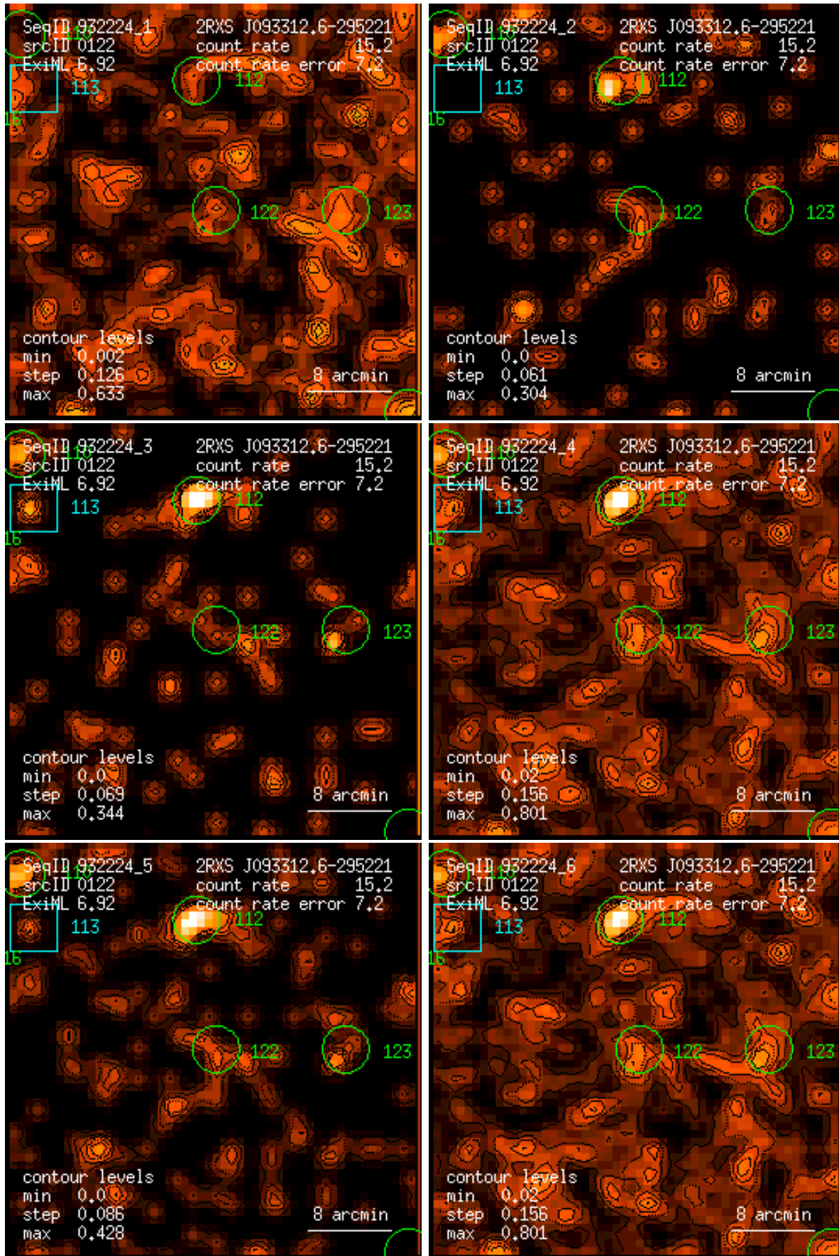
Figure 122: RASS 932224: detection 0122: band rate images, Gaussian filter: (1) PSPC channels 11 – 41, (2) 52 – 90, (3) 91 – 201, (4) 11 – 235, (5) 52 – 201, (6) 11 – 201. Broad band rates in counts/ks. Band rate contour levels in counts/ks/arcmin 2 .
