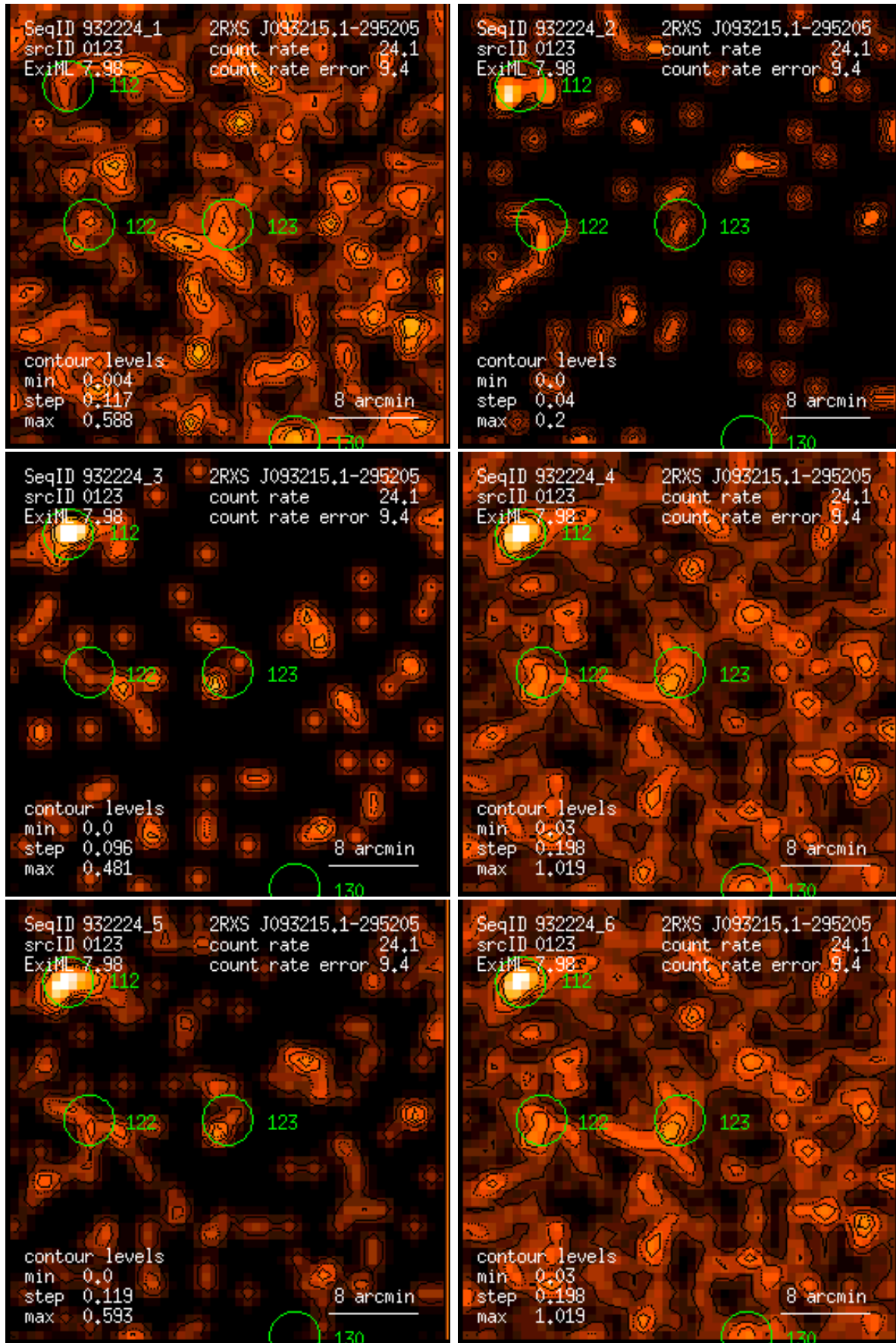
Figure 123: RASS 932224: detection 0123: band rate images, Gaussian filter: (1) PSPC channels 11 – 41, (2) 52 – 90, (3) 91 – 201, (4) 11 – 235, (5) 52 – 201, (6) 11 – 201. Broad band rates in counts/ks. Band rate contour levels in counts/ks/arcmin 2 .
