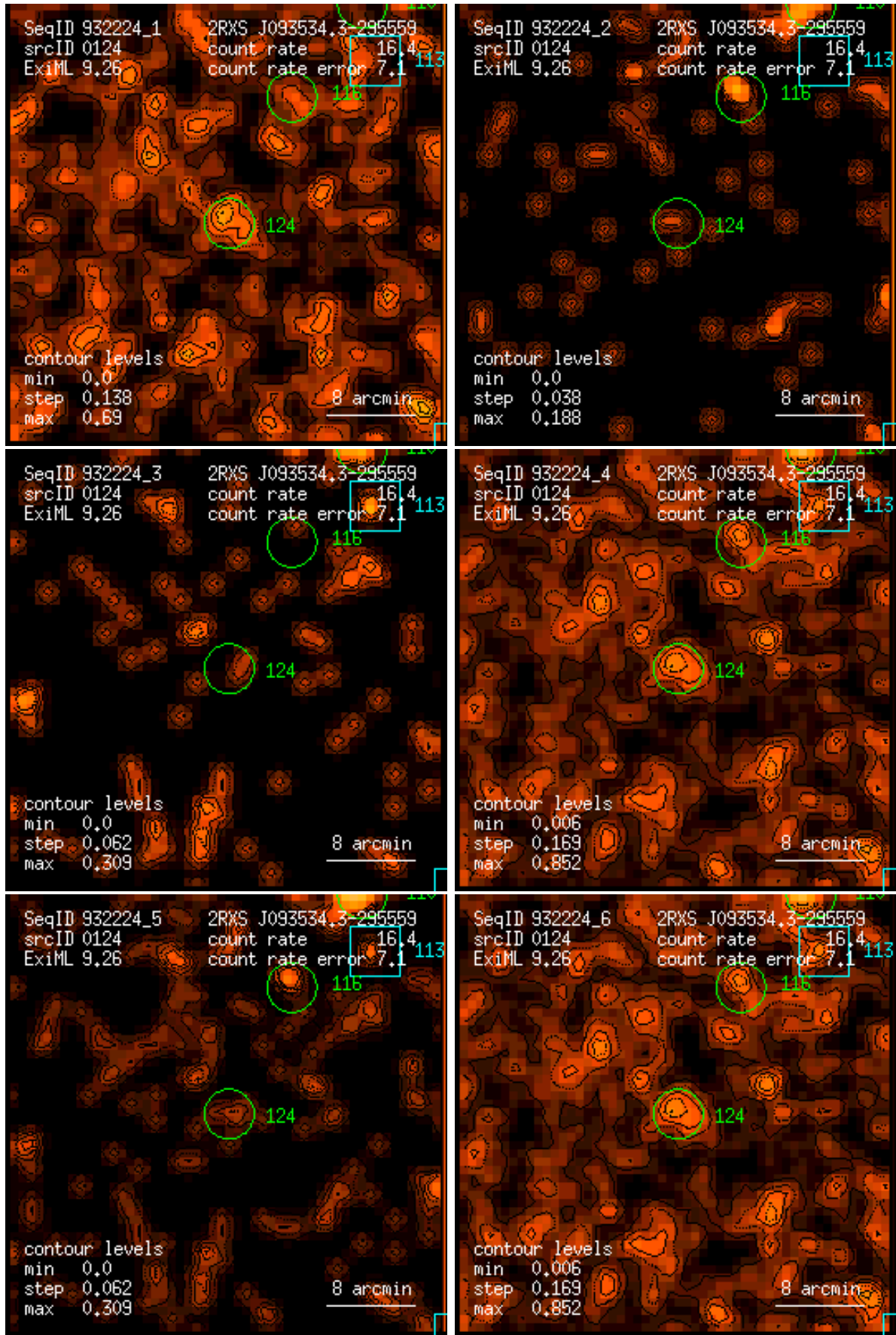
Figure 124: RASS 932224: detection 0124: band rate images, Gaussian filter: (1) PSPC channels 11 – 41, (2) 52 – 90, (3) 91 – 201, (4) 11 – 235, (5) 52 – 201, (6) 11 – 201. Broad band rates in counts/ks. Band rate contour levels in counts/ks/arcmin 2 .
