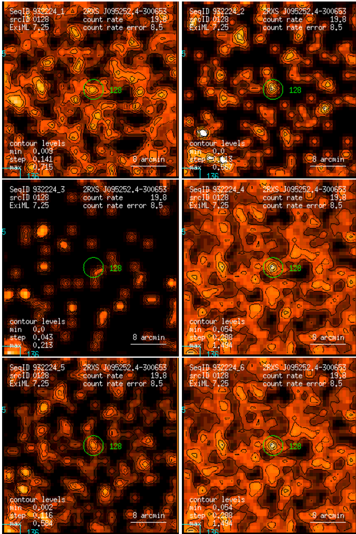
Figure 128: RASS 932224: detection 0128: band rate images, Gaussian filter: (1) PSPC channels 11 – 41, (2) 52 – 90, (3) 91 – 201, (4) 11 – 235, (5) 52 – 201, (6) 11 – 201. Broad band rates in counts/ks. Band rate contour levels in counts/ks/arcmin 2 .
