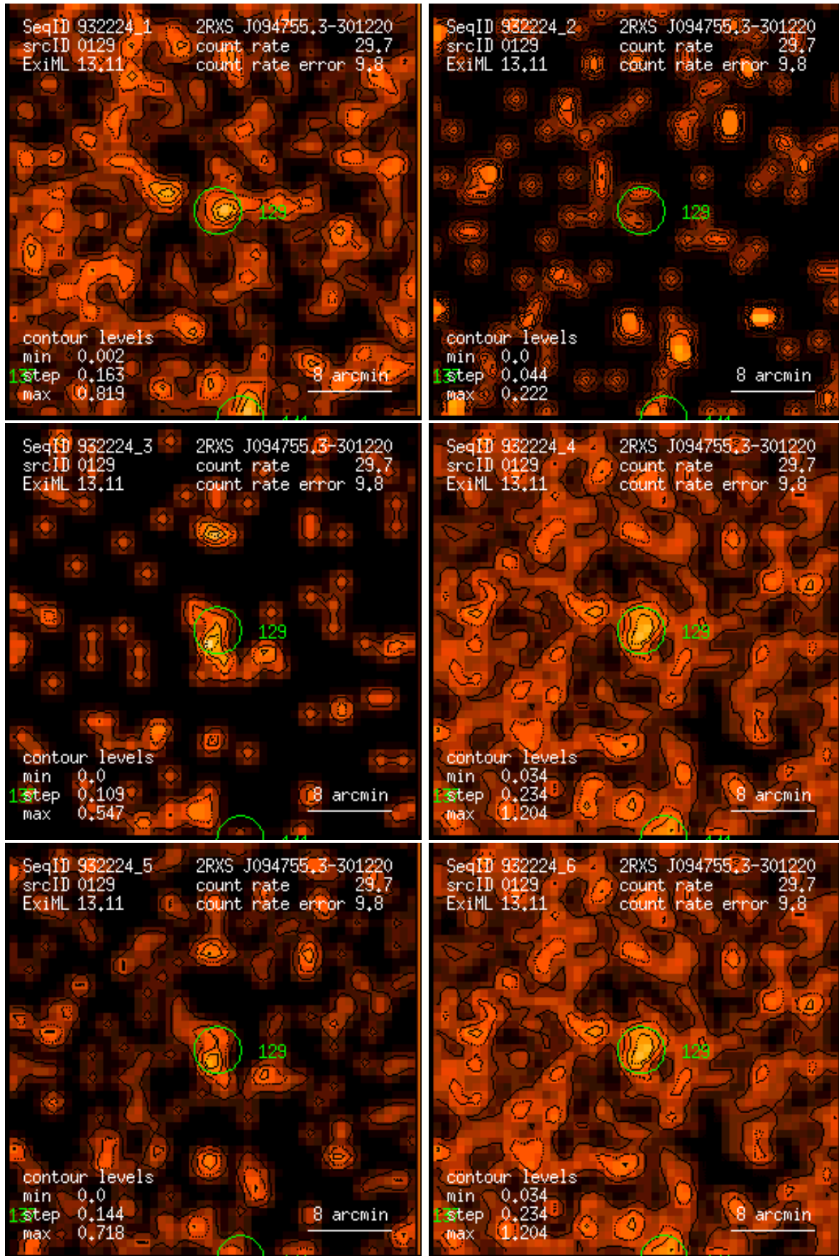
Figure 129: RASS 932224: detection 0129: band rate images, Gaussian filter: (1) PSPC channels 11 – 41, (2) 52 – 90, (3) 91 – 201, (4) 11 – 235, (5) 52 – 201, (6) 11 – 201. Broad band rates in counts/ks. Band rate contour levels in counts/ks/arcmin 2 .
