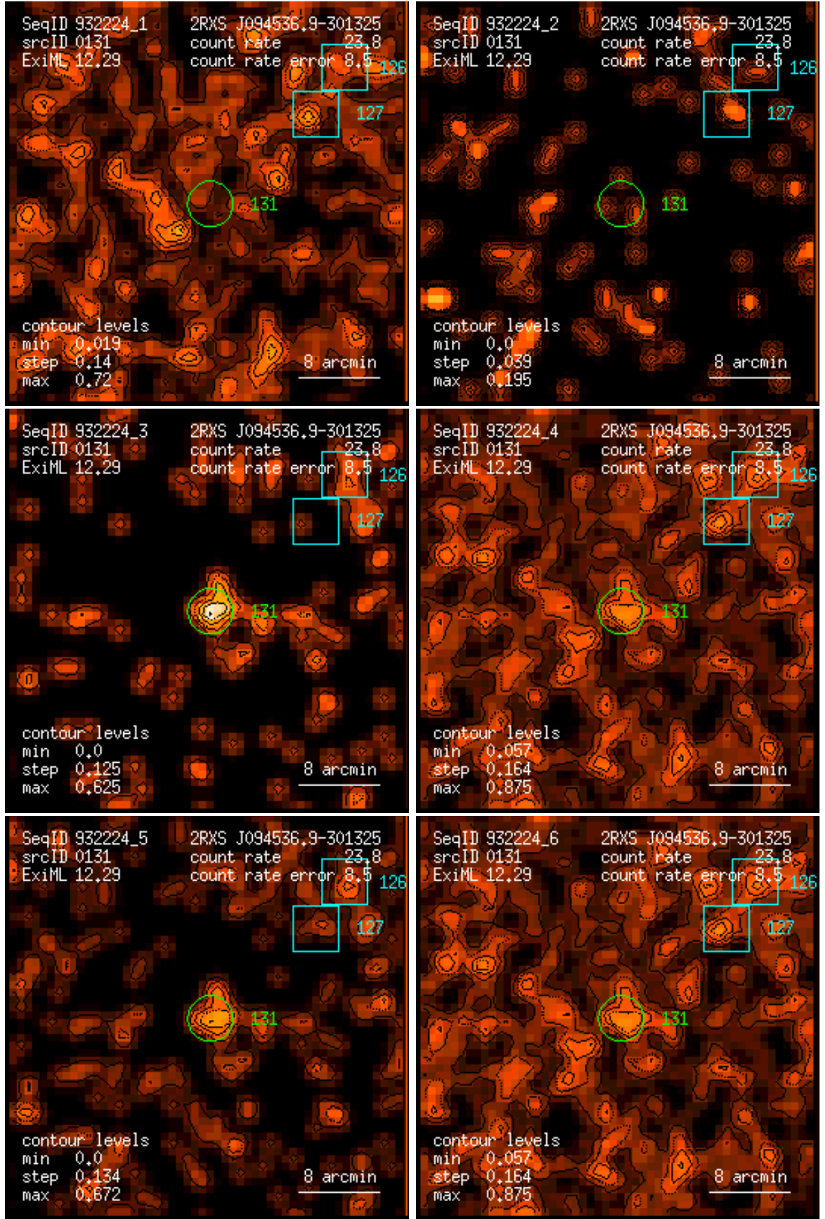
Figure 131: RASS 932224: detection 0131: band rate images, Gaussian filter: (1) PSPC channels 11 – 41, (2) 52 – 90, (3) 91 – 201, (4) 11 – 235, (5) 52 – 201, (6) 11 – 201. Broad band rates in counts/ks. Band rate contour levels in counts/ks/arcmin 2 .
