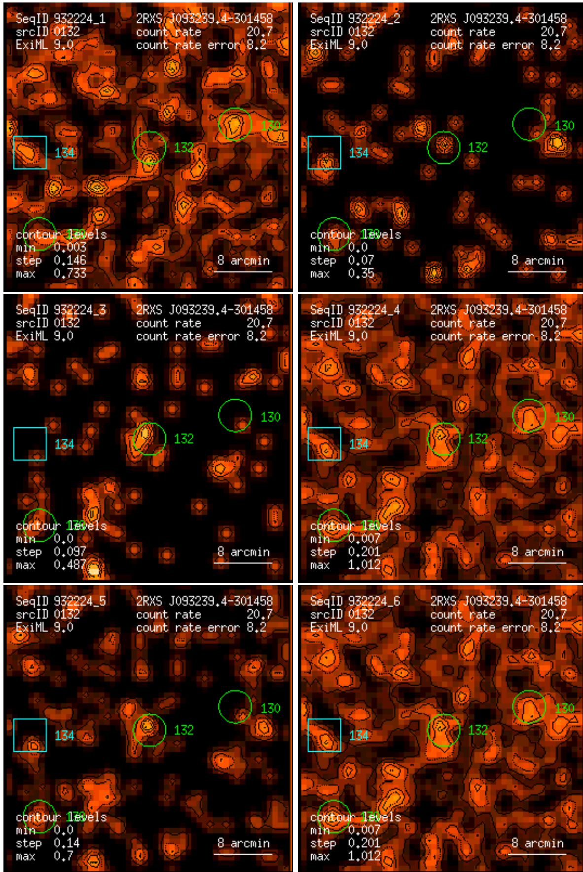
Figure 132: RASS 932224: detection 0132: band rate images, Gaussian filter: (1) PSPC channels 11 – 41, (2) 52 – 90, (3) 91 – 201, (4) 11 – 235, (5) 52 – 201, (6) 11 – 201. Broad band rates in counts/ks. Band rate contour levels in counts/ks/arcmin 2 .
