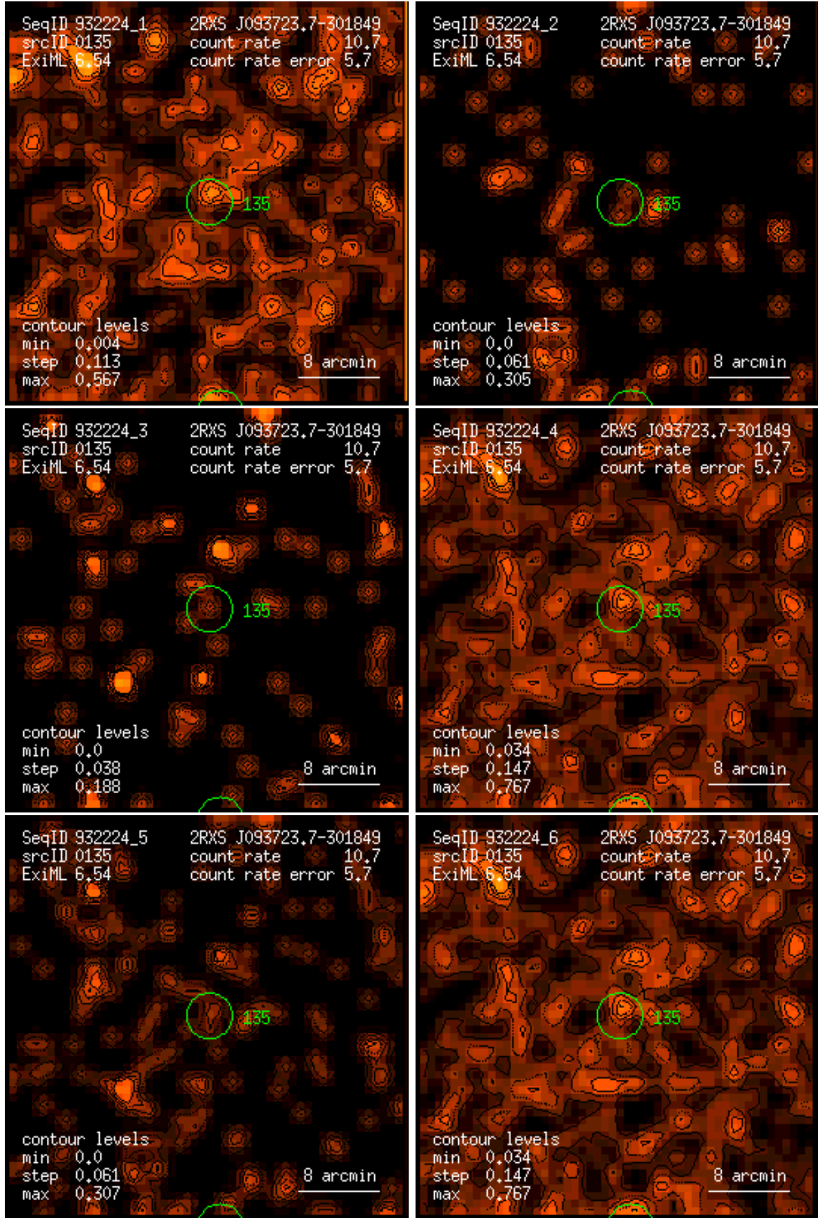
Figure 135: RASS 932224: detection 0135: band rate images, Gaussian filter: (1) PSPC channels 11 – 41, (2) 52 – 90, (3) 91 – 201, (4) 11 – 235, (5) 52 – 201, (6) 11 – 201. Broad band rates in counts/ks. Band rate contour levels in counts/ks/arcmin 2 .
