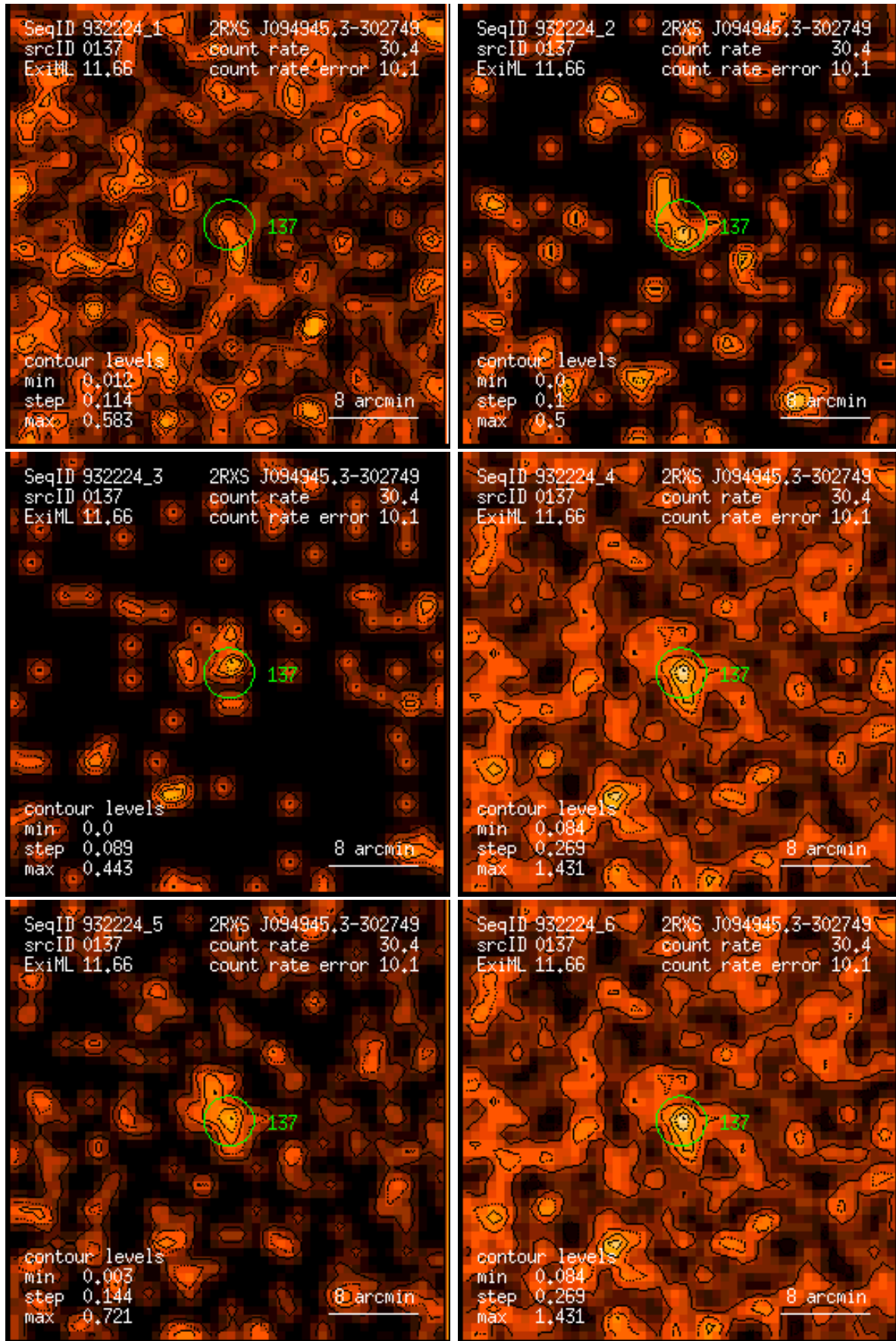
Figure 137: RASS 932224: detection 0137: band rate images, Gaussian filter: (1) PSPC channels 11 – 41, (2) 52 – 90, (3) 91 – 201, (4) 11 – 235, (5) 52 – 201, (6) 11 – 201. Broad band rates in counts/ks. Band rate contour levels in counts/ks/arcmin 2 .
