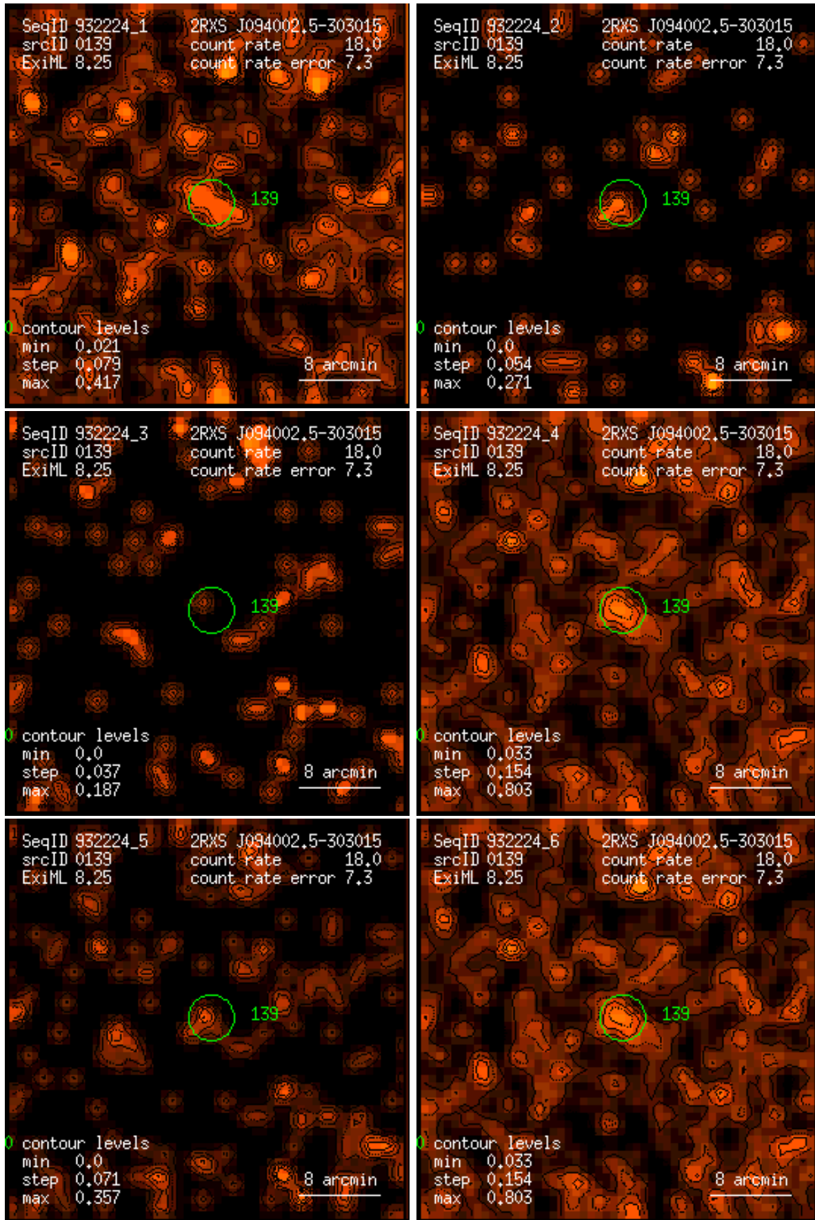
Figure 139: RASS 932224: detection 0139: band rate images, Gaussian filter: (1) PSPC channels 11 – 41, (2) 52 – 90, (3) 91 – 201, (4) 11 – 235, (5) 52 – 201, (6) 11 – 201. Broad band rates in counts/ks. Band rate contour levels in counts/ks/arcmin 2 .
