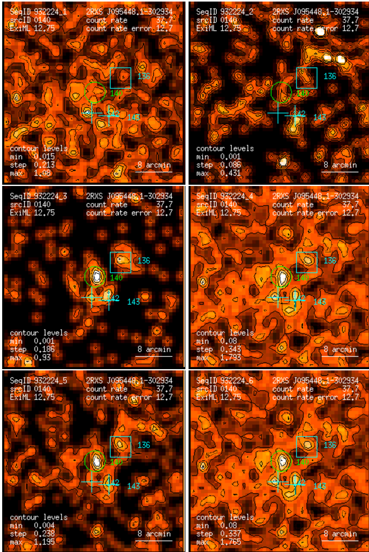
Figure 140: RASS 932224: detection 0140: band rate images, Gaussian filter: (1) PSPC channels 11 – 41, (2) 52 – 90, (3) 91 – 201, (4) 11 – 235, (5) 52 – 201, (6) 11 – 201. Broad band rates in counts/ks. Band rate contour levels in counts/ks/arcmin 2 .
