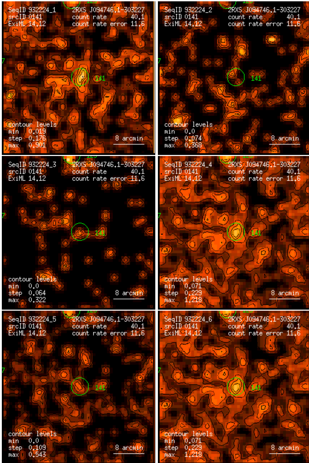
Figure 141: RASS 932224: detection 0141: band rate images, Gaussian filter: (1) PSPC channels 11 – 41, (2) 52 – 90, (3) 91 – 201, (4) 11 – 235, (5) 52 – 201, (6) 11 – 201. Broad band rates in counts/ks. Band rate contour levels in counts/ks/arcmin 2 .
