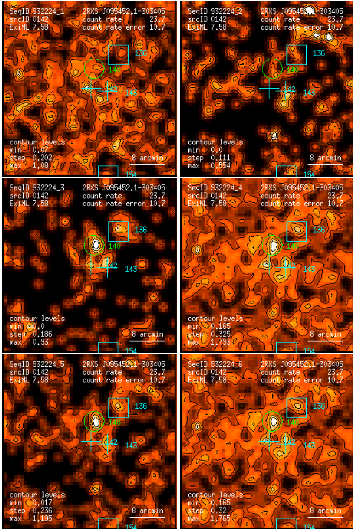
Figure 142: RASS 932224: detection 0142: band rate images, Gaussian filter: (1) PSPC channels 11 – 41, (2) 52 – 90, (3) 91 – 201, (4) 11 – 235, (5) 52 – 201, (6) 11 – 201. Broad band rates in counts/ks. Band rate contour levels in counts/ks/arcmin 2 .
