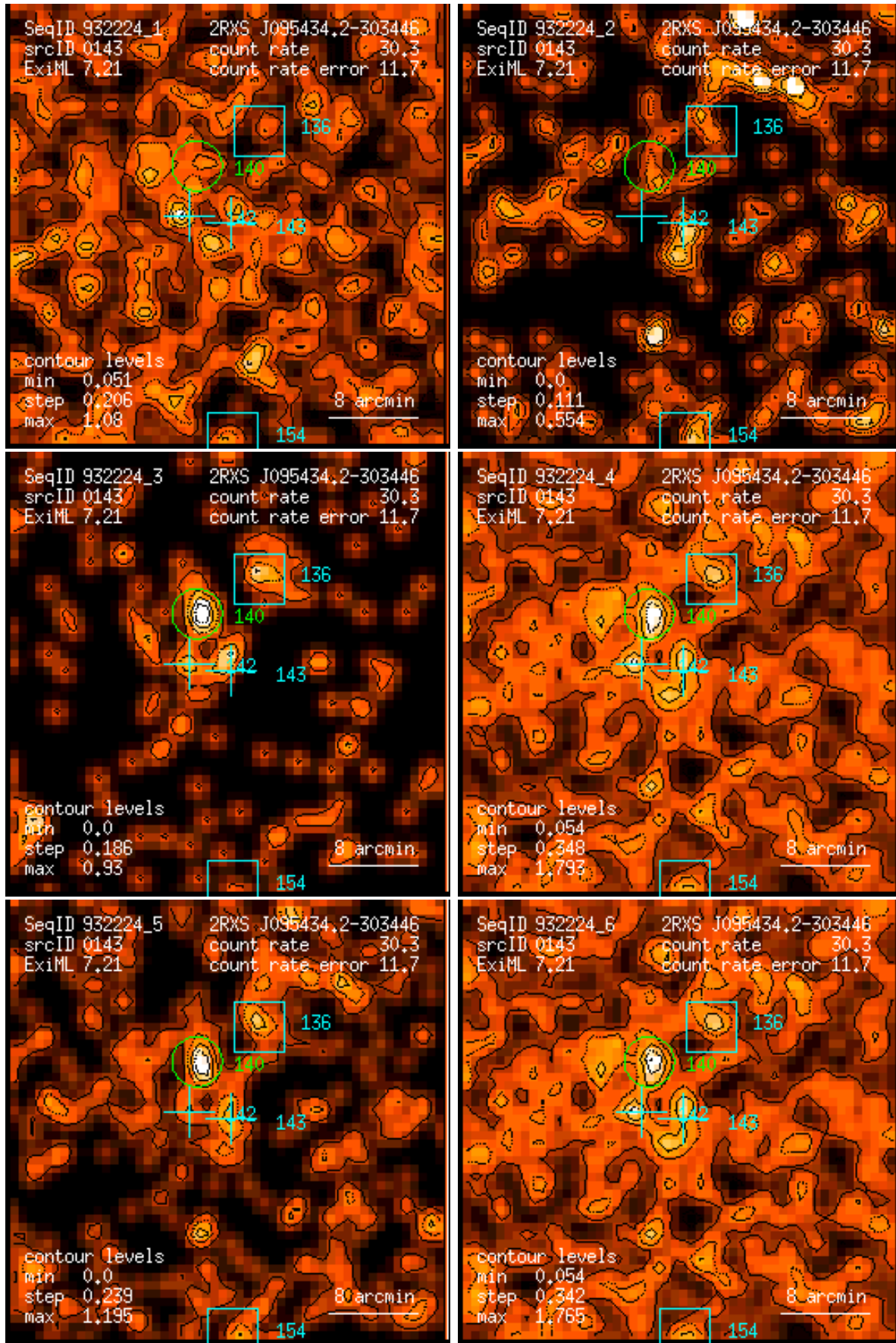
Figure 143: RASS 932224: detection 0143: band rate images, Gaussian filter: (1) PSPC channels 11 – 41, (2) 52 – 90, (3) 91 – 201, (4) 11 – 235, (5) 52 – 201, (6) 11 – 201. Broad band rates in counts/ks. Band rate contour levels in counts/ks/arcmin 2 .
