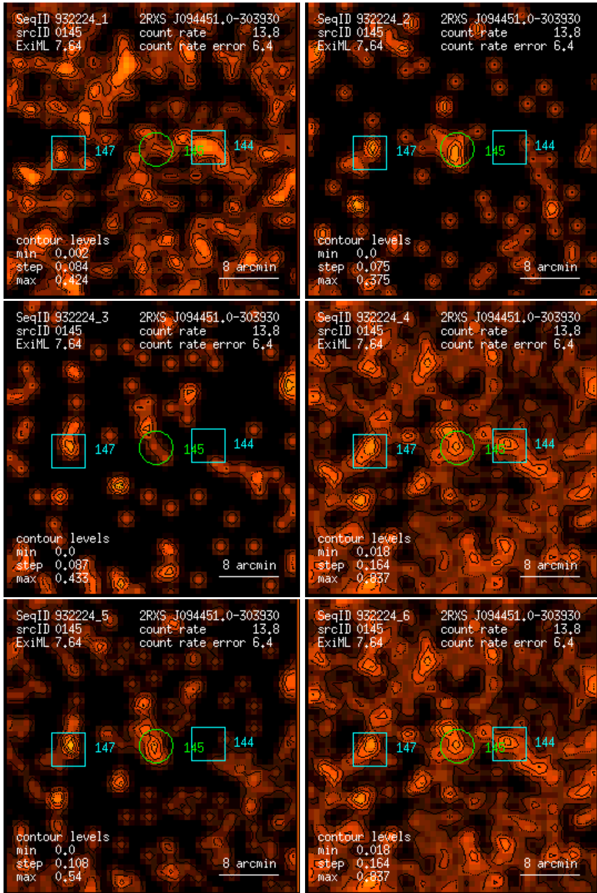
Figure 145: RASS 932224: detection 0145: band rate images, Gaussian filter: (1) PSPC channels 11 – 41, (2) 52 – 90, (3) 91 – 201, (4) 11 – 235, (5) 52 – 201, (6) 11 – 201. Broad band rates in counts/ks. Band rate contour levels in counts/ks/arcmin 2 .
