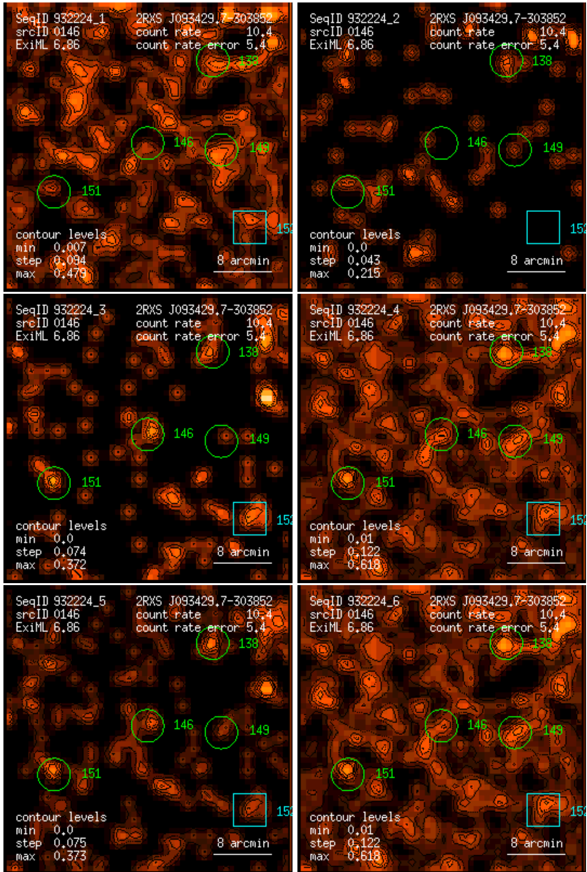
Figure 146: RASS 932224: detection 0146: band rate images, Gaussian filter: (1) PSPC channels 11 – 41, (2) 52 – 90, (3) 91 – 201, (4) 11 – 235, (5) 52 – 201, (6) 11 – 201. Broad band rates in counts/ks. Band rate contour levels in counts/ks/arcmin 2 .
