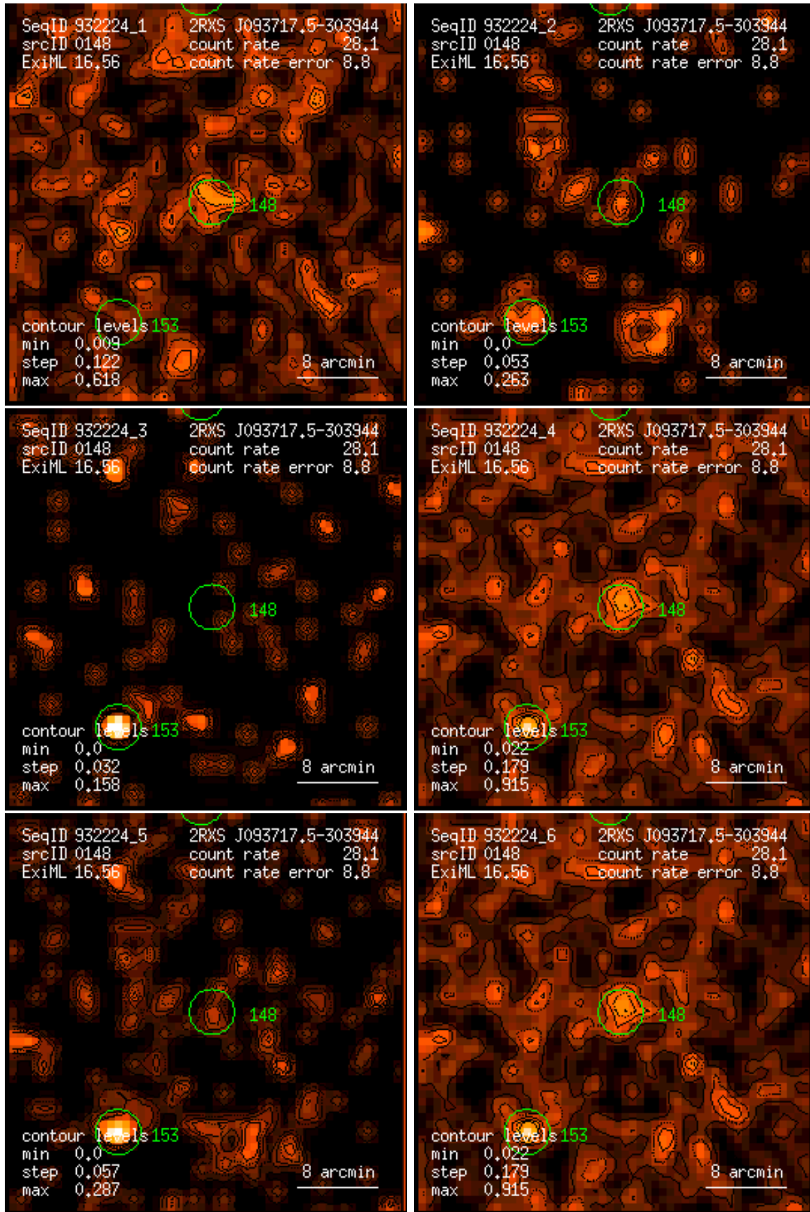
Figure 148: RASS 932224: detection 0148: band rate images, Gaussian filter: (1) PSPC channels 11 – 41, (2) 52 – 90, (3) 91 – 201, (4) 11 – 235, (5) 52 – 201, (6) 11 – 201. Broad band rates in counts/ks. Band rate contour levels in counts/ks/arcmin 2 .
