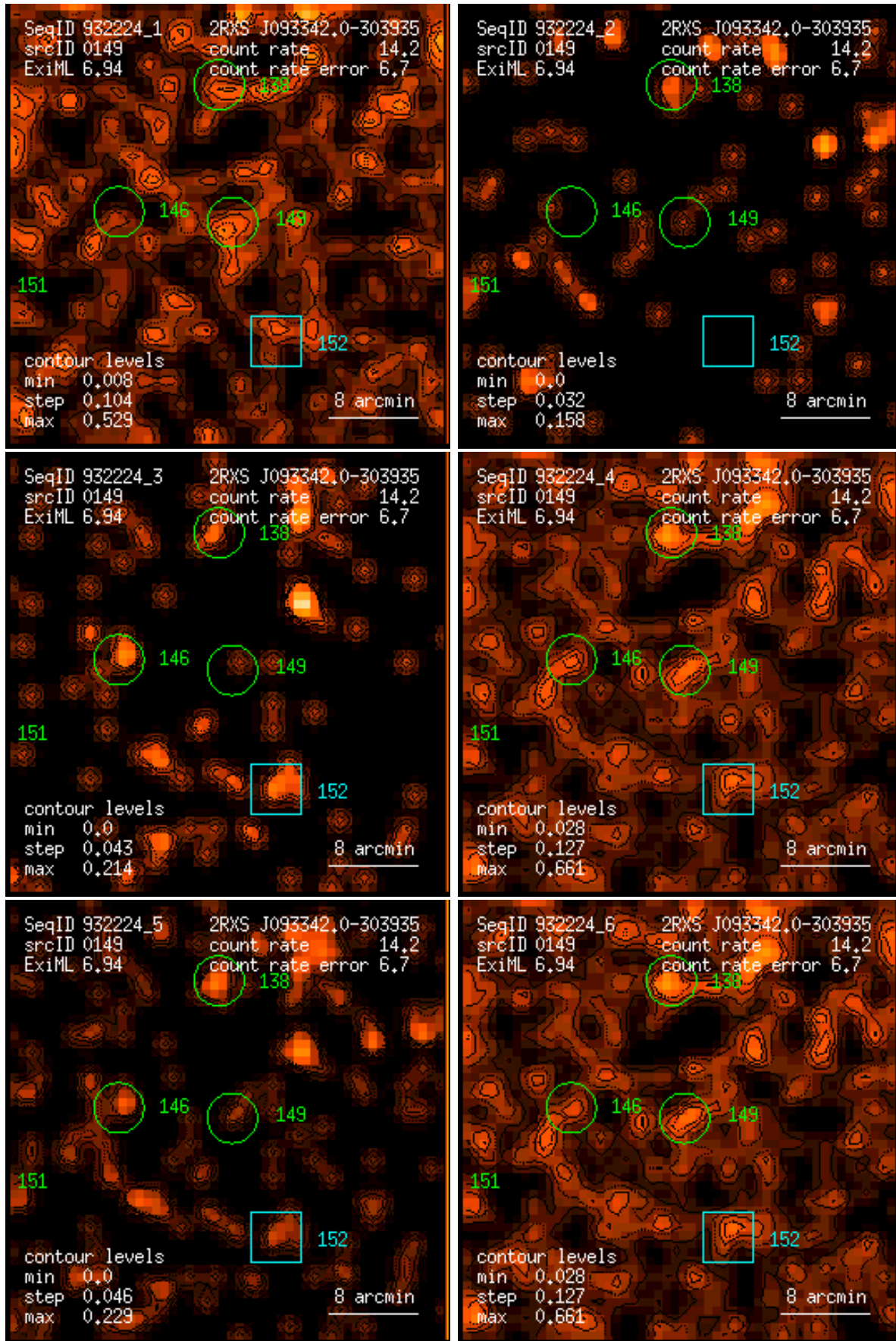
Figure 149: RASS 932224: detection 0149: band rate images, Gaussian filter: (1) PSPC channels 11 – 41, (2) 52 – 90, (3) 91 – 201, (4) 11 – 235, (5) 52 – 201, (6) 11 – 201. Broad band rates in counts/ks. Band rate contour levels in counts/ks/arcmin 2 .
