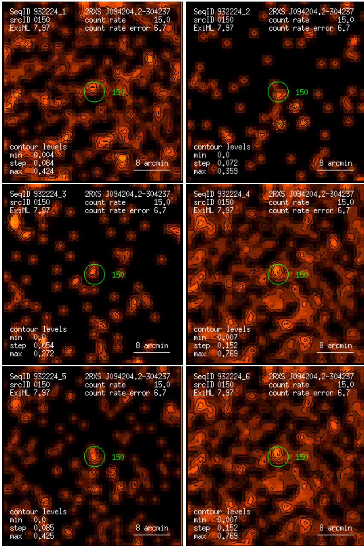
Figure 150: RASS 932224: detection 0150: band rate images, Gaussian filter: (1) PSPC channels 11 – 41, (2) 52 – 90, (3) 91 – 201, (4) 11 – 235, (5) 52 – 201, (6) 11 – 201. Broad band rates in counts/ks. Band rate contour levels in counts/ks/arcmin 2 .
