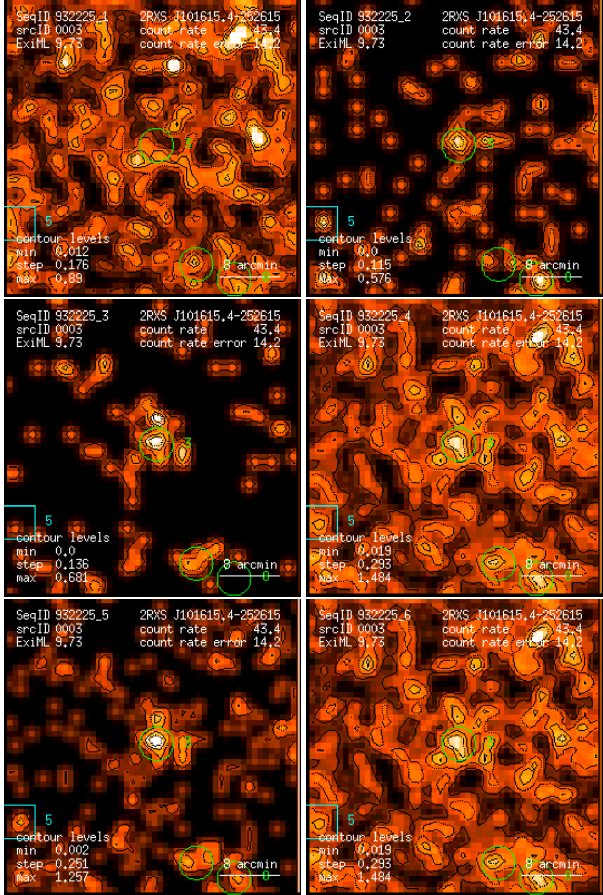
Figure 3: RASS 932225: detection 0003: band rate images, Gaussian filter: (1) PSPC channels 11 – 41, (2) 52 – 90, (3) 91 – 201, (4) 11 – 235, (5) 52 – 201, (6) 11 – 201. Broad band rates in counts/ks. Band rate contour levels in counts/ks/arcmin 2 .
