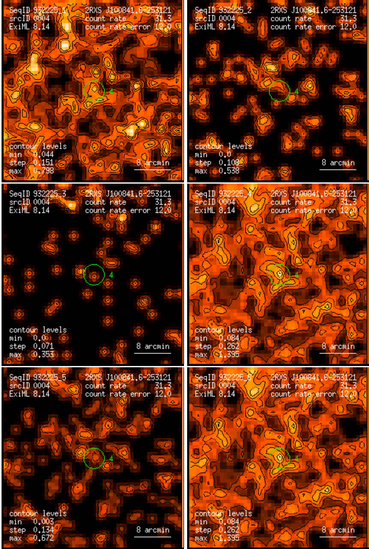
Figure 4: RASS 932225: detection 0004: band rate images, Gaussian filter: (1) PSPC channels 11 – 41, (2) 52 – 90, (3) 91 – 201, (4) 11 – 235, (5) 52 – 201, (6) 11 – 201. Broad band rates in counts/ks. Band rate contour levels in counts/ks/arcmin 2 .
