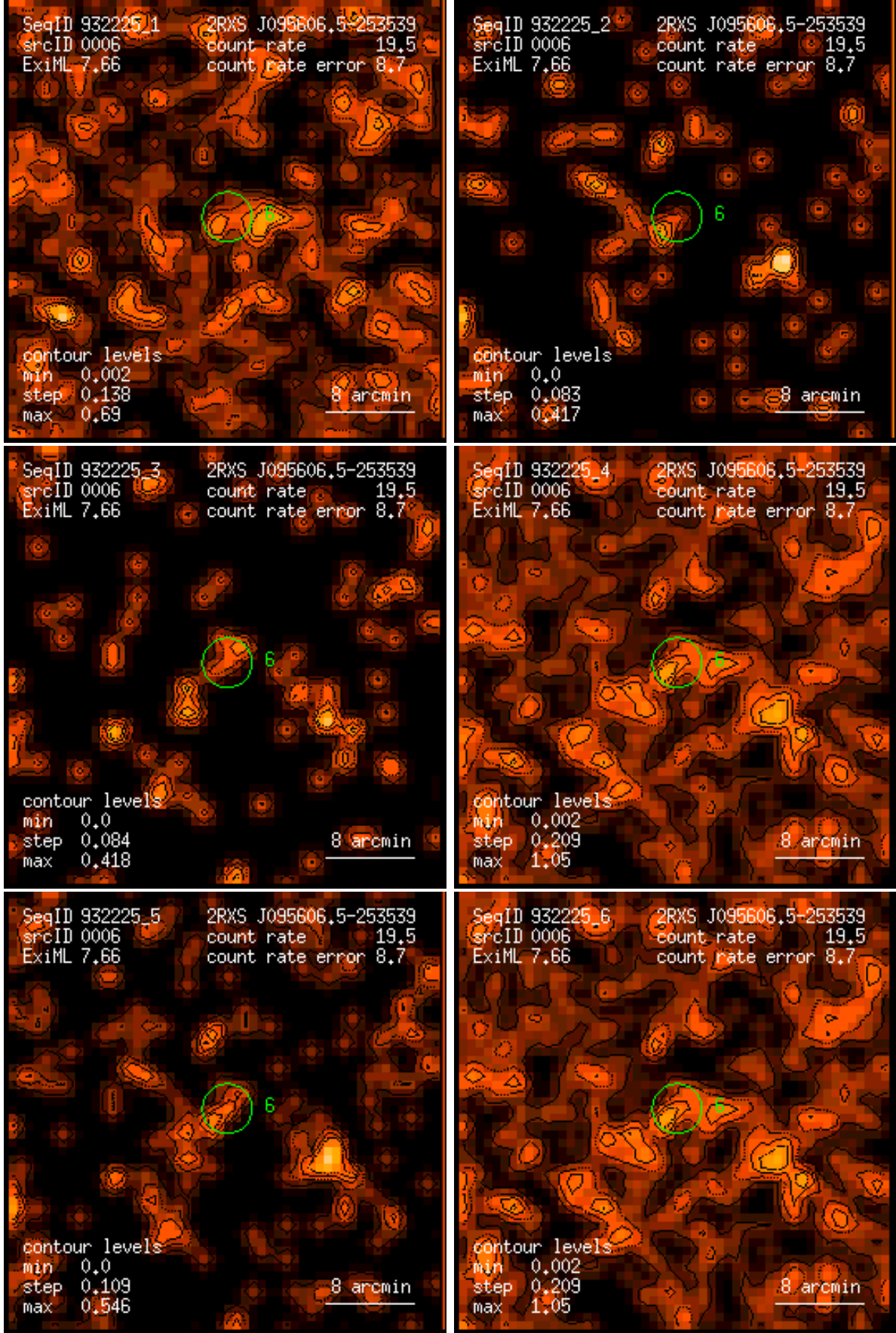
Figure 6: RASS 932225: detection 0006: band rate images, Gaussian filter: (1) PSPC channels 11 – 41, (2) 52 – 90, (3) 91 – 201, (4) 11 – 235, (5) 52 – 201, (6) 11 – 201. Broad band rates in counts/ks. Band rate contour levels in counts/ks/arcmin 2 .
