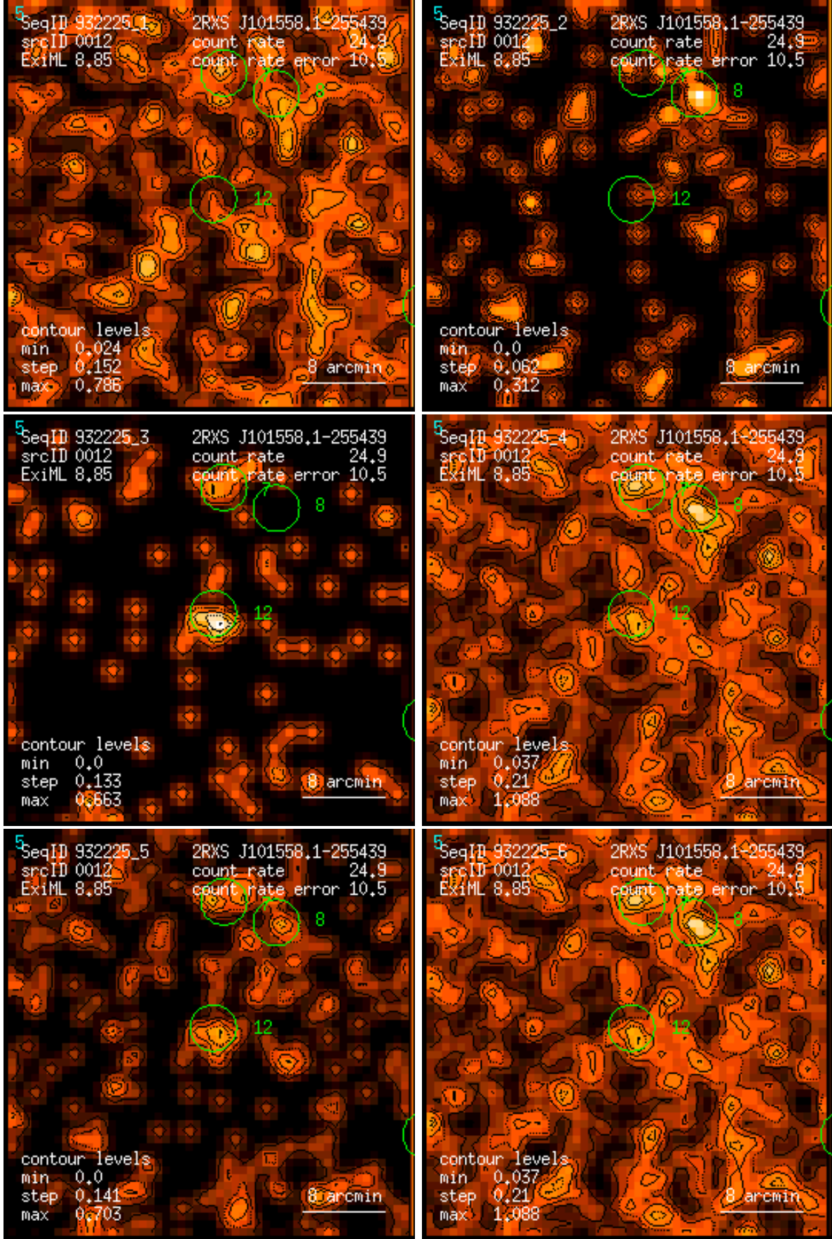
Figure 12: RASS 932225: detection 0012: band rate images, Gaussian filter: (1) PSPC channels 11 – 41, (2) 52 – 90, (3) 91 – 201, (4) 11 – 235, (5) 52 – 201, (6) 11 – 201. Broad band rates in counts/ks. Band rate contour levels in counts/ks/arcmin 2 .
