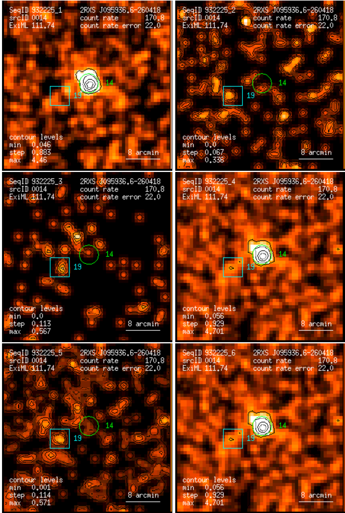
Figure 14: RASS 932225: detection 0014: band rate images, Gaussian filter: (1) PSPC channels 11 – 41, (2) 52 – 90, (3) 91 – 201, (4) 11 – 235, (5) 52 – 201, (6) 11 – 201. Broad band rates in counts/ks. Band rate contour levels in counts/ks/arcmin 2 .
