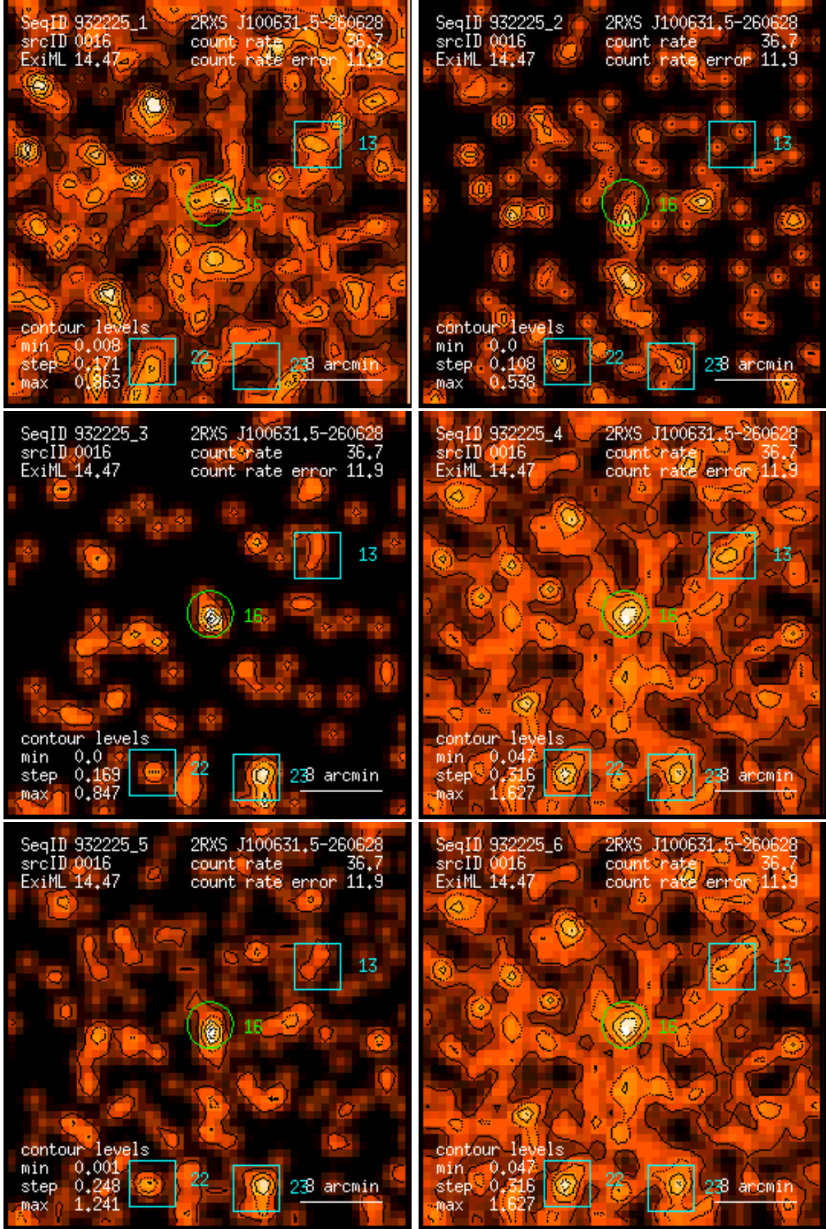
Figure 16: RASS 932225: detection 0016: band rate images, Gaussian filter: (1) PSPC channels 11 – 41, (2) 52 – 90, (3) 91 – 201, (4) 11 – 235, (5) 52 – 201, (6) 11 – 201. Broad band rates in counts/ks. Band rate contour levels in counts/ks/arcmin 2 .
