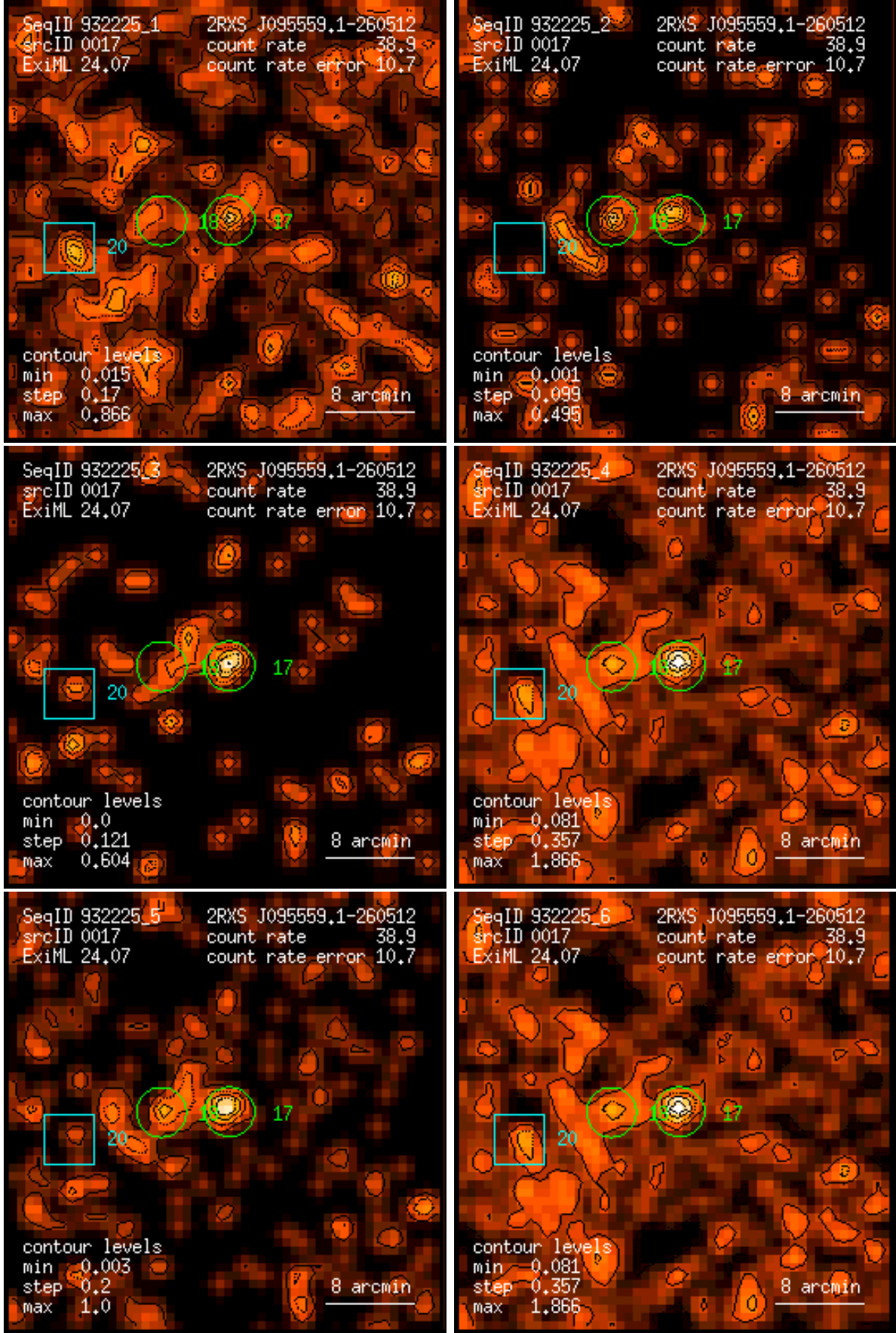
Figure 17: RASS 932225: detection 0017: band rate images, Gaussian filter: (1) PSPC channels 11 – 41, (2) 52 – 90, (3) 91 – 201, (4) 11 – 235, (5) 52 – 201, (6) 11 – 201. Broad band rates in counts/ks. Band rate contour levels in counts/ks/arcmin 2 .
