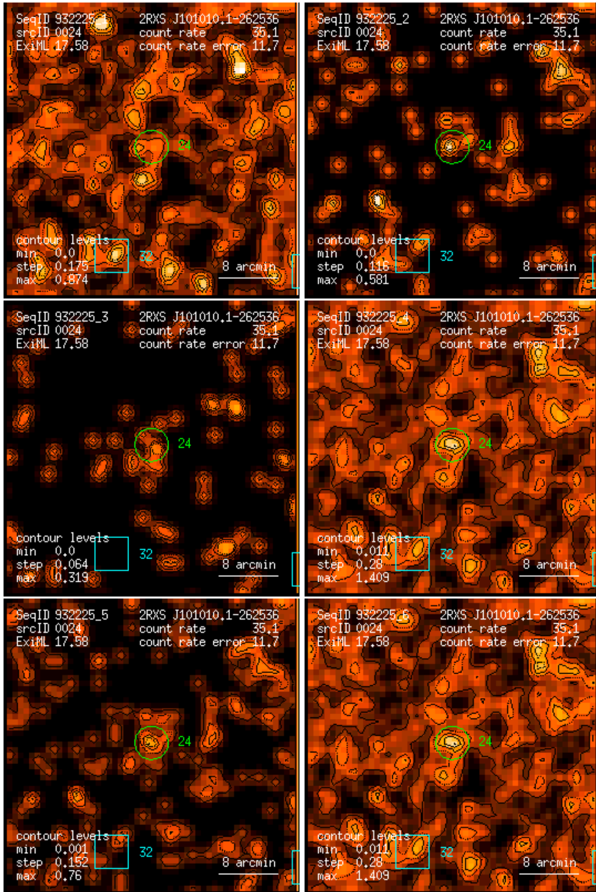
Figure 24: RASS 932225: detection 0024: band rate images, Gaussian filter: (1) PSPC channels 11 – 41, (2) 52 – 90, (3) 91 – 201, (4) 11 – 235, (5) 52 – 201, (6) 11 – 201. Broad band rates in counts/ks. Band rate contour levels in counts/ks/arcmin 2 .
