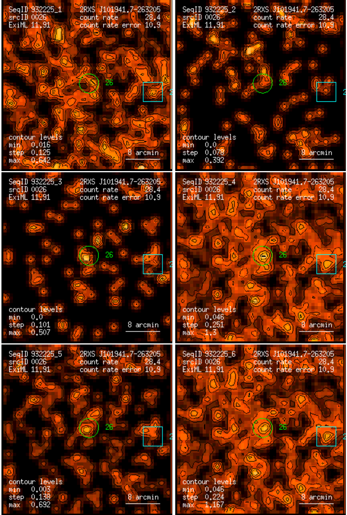
Figure 26: RASS 932225: detection 0026: band rate images, Gaussian filter: (1) PSPC channels 11 – 41, (2) 52 – 90, (3) 91 – 201, (4) 11 – 235, (5) 52 – 201, (6) 11 – 201. Broad band rates in counts/ks. Band rate contour levels in counts/ks/arcmin 2 .
