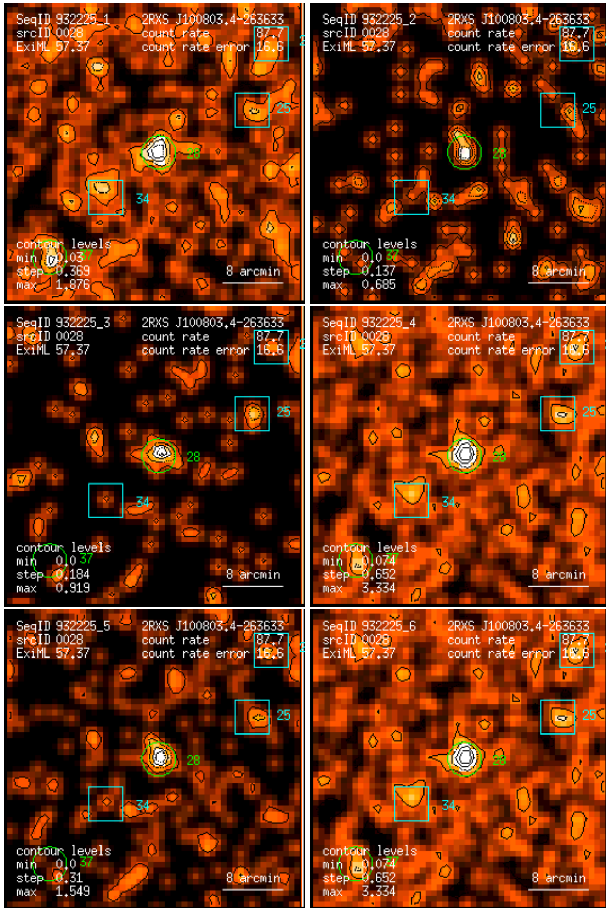
Figure 28: RASS 932225: detection 0028: band rate images, Gaussian filter: (1) PSPC channels 11 – 41, (2) 52 – 90, (3) 91 – 201, (4) 11 – 235, (5) 52 – 201, (6) 11 – 201. Broad band rates in counts/ks. Band rate contour levels in counts/ks/arcmin 2 .
